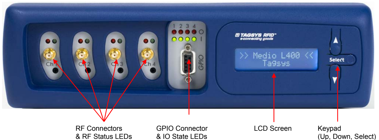
Figure 1: Front panel
