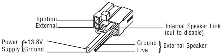
Figure 5: Power Connector Wiring
