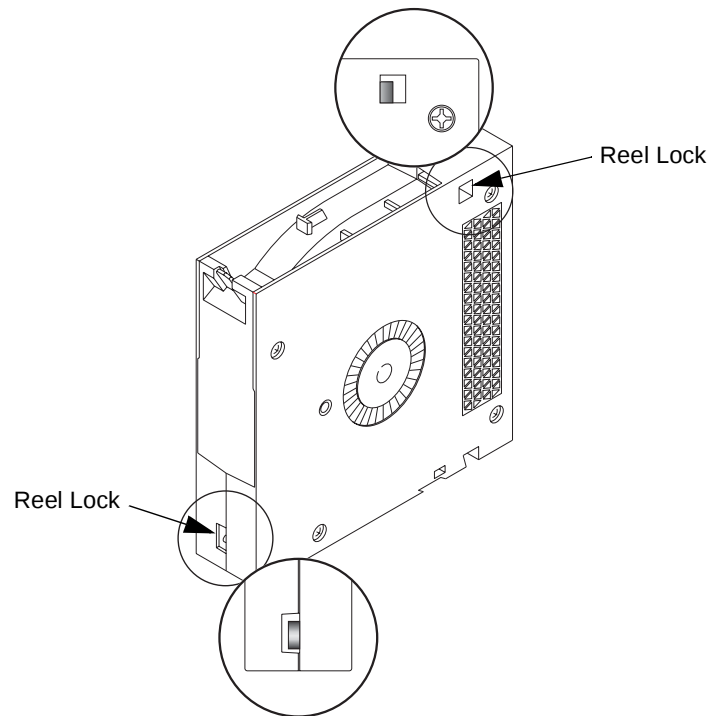
Figure B-2. DLTtape VS1 Data Cartridge Reel Locks
