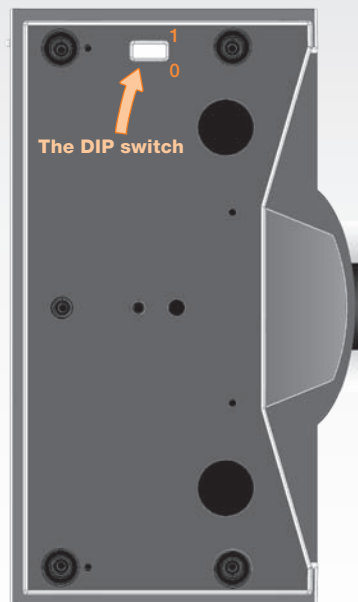
Underside side of the TANDBERG PrecisionHD 1080p camera
