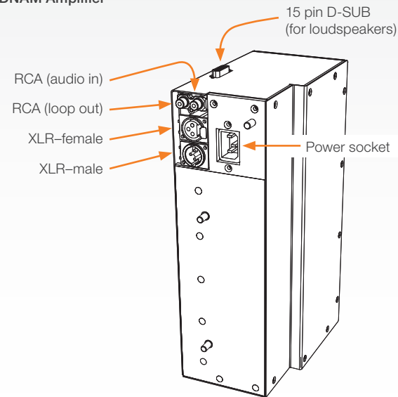
DNAM Amplifier
