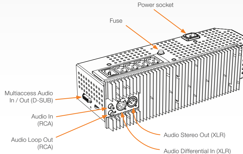
DNAM Amplifier
