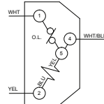
GE/RBC BEATER MOTOR "CW" ROTATION (SEE NOTE #1)
