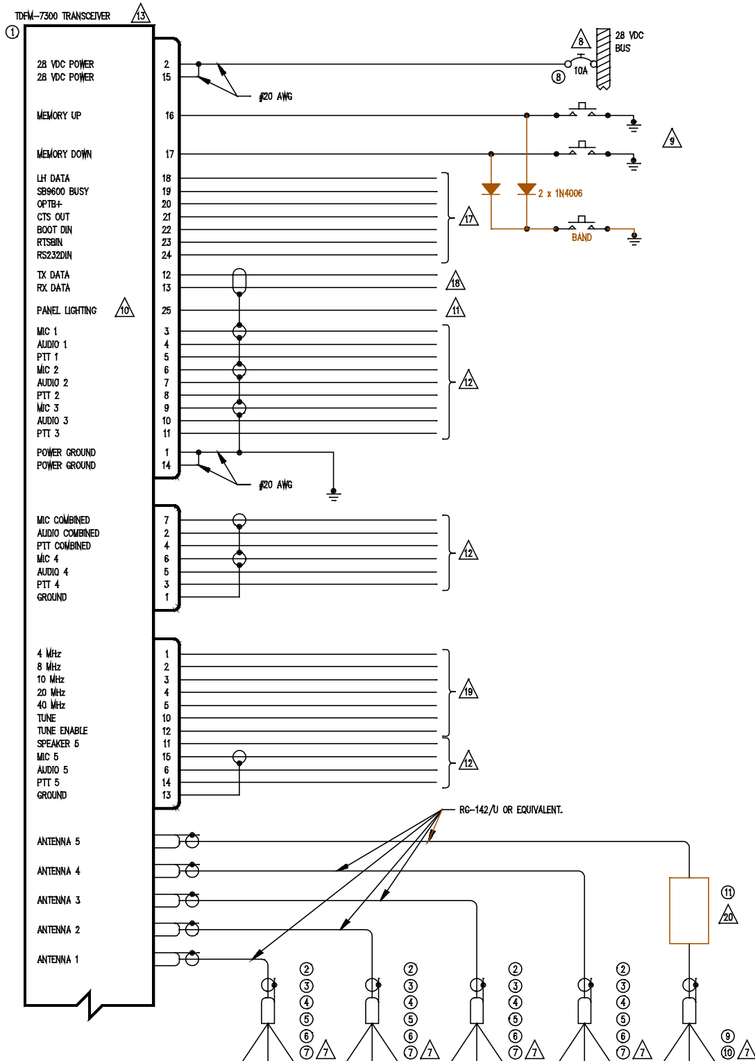
FIGURE 3-2a Wiring connections for the TDFM-7300-3 Transceiver
