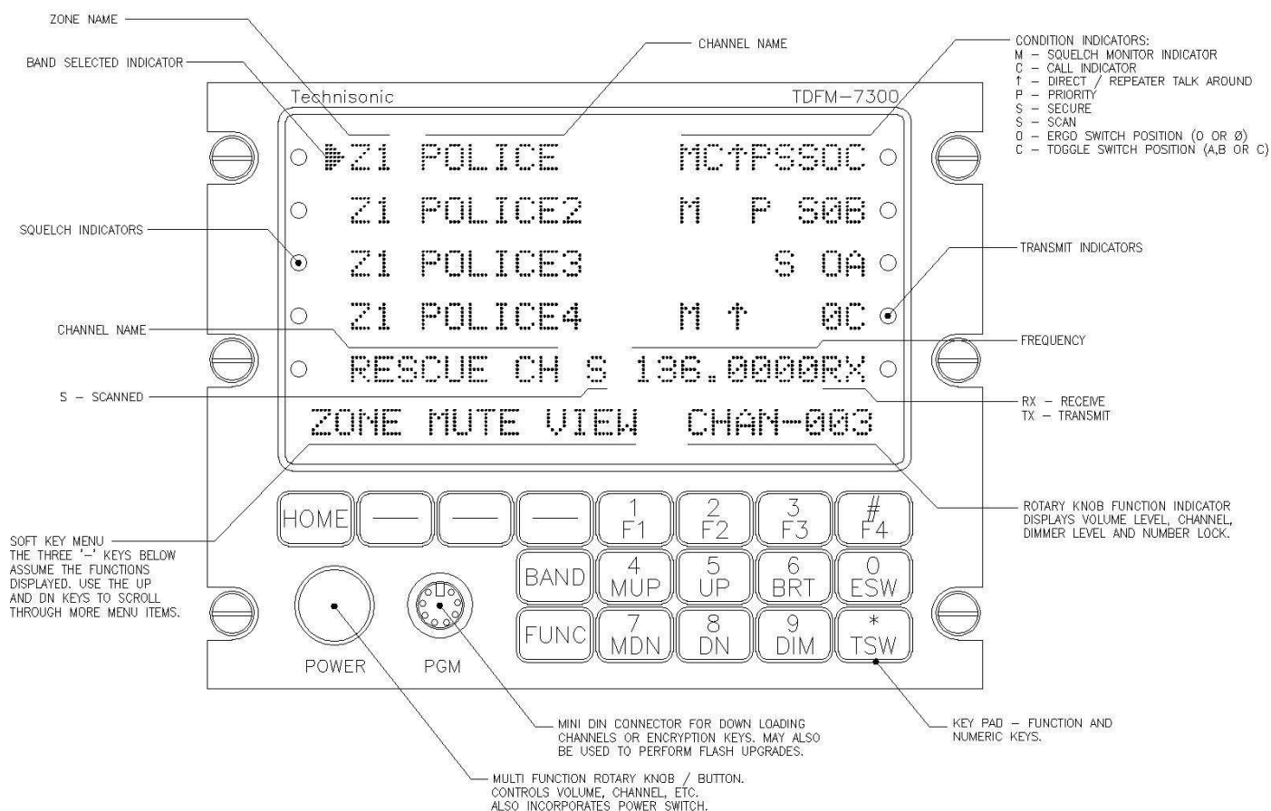
FIGURE 2-1 Front Panel Controls – TDFM-7300-3 Transceiver
