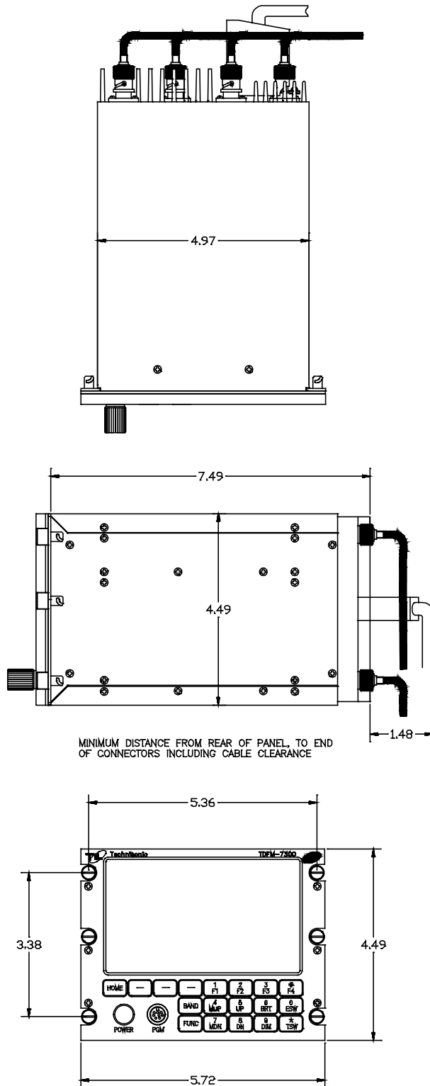
FIGURE 3-1 Outline Drawing for Model TDFM-7300-3
