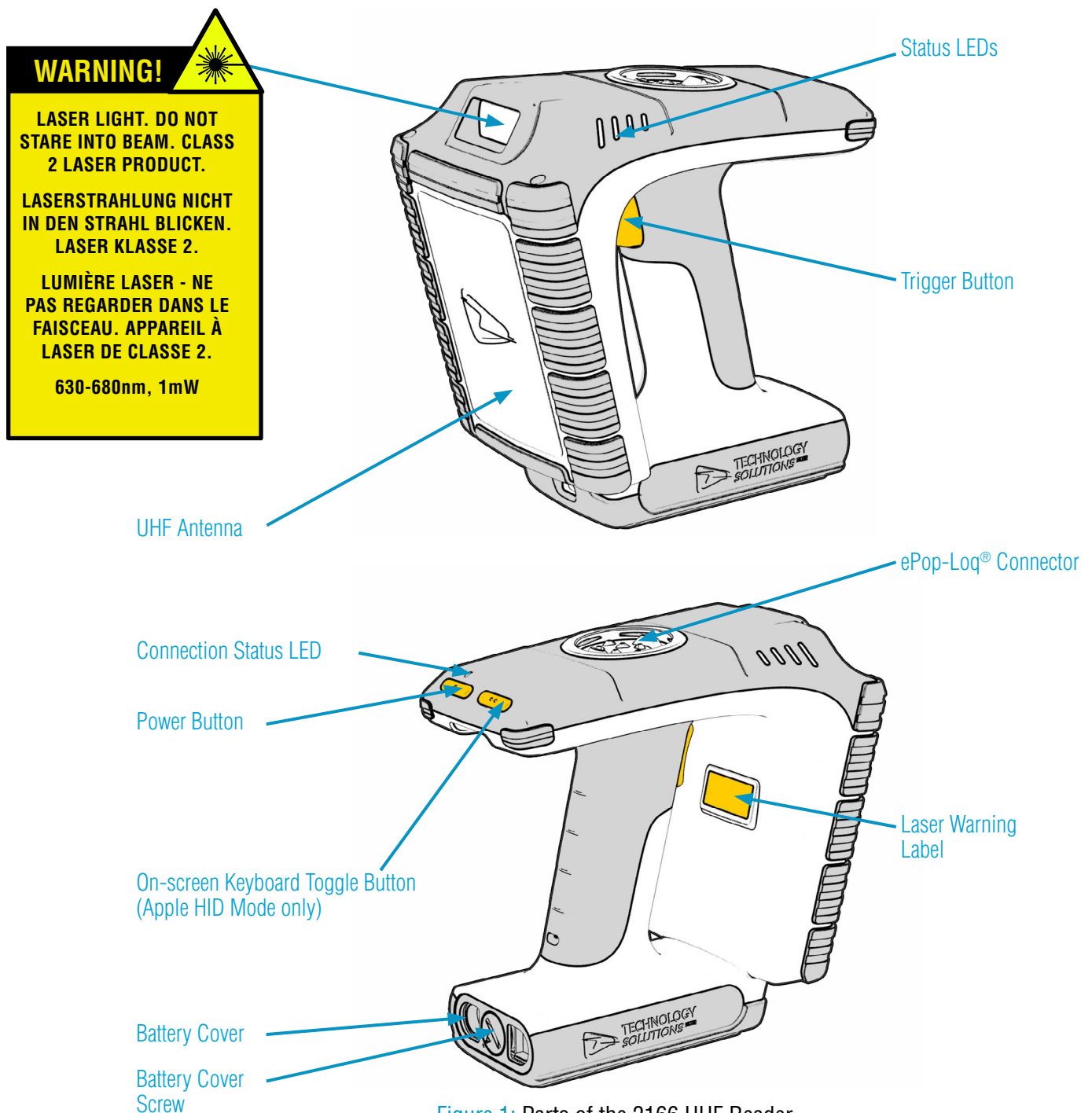
Figure 1: Parts of the 2166 UHF Reader
