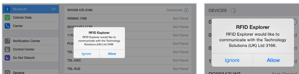
Figure 14: Allow connection
