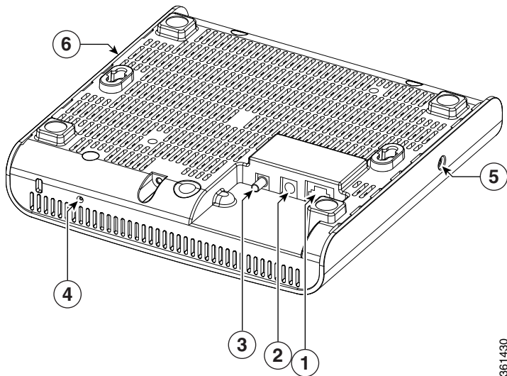
Figure 2 Cisco USC 7330 Connections
