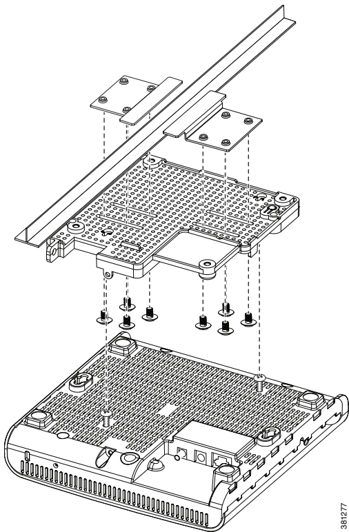
Figure 4 Cisco USC 7330 with Suspended Ceiling Bracket
