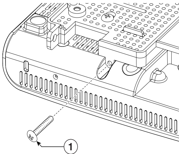
Figure 5 Suspended Ceiling Bracket with Locking Screw
