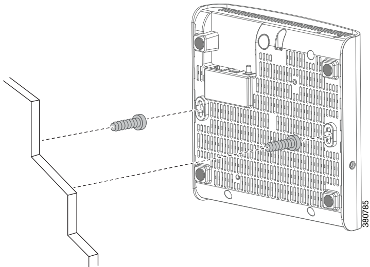
Figure 3 Cisco USC 7330 Mounted Vertically on Wall
