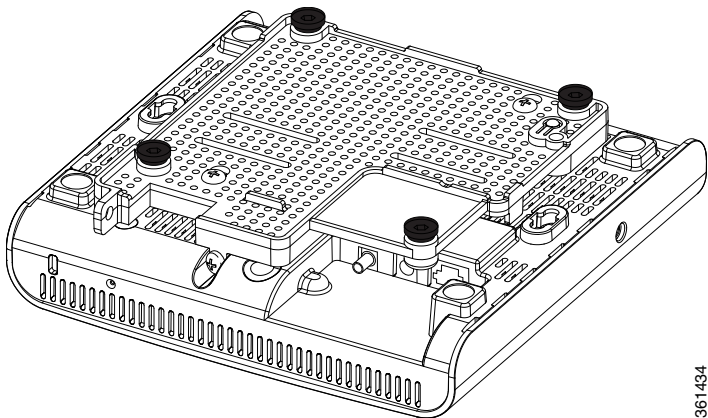
Figure 6 Suspended Ceiling Bracket with Attached Feet
