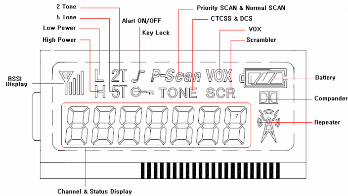
Figure 3-2) XV/XU-100 Series LCD Indication
