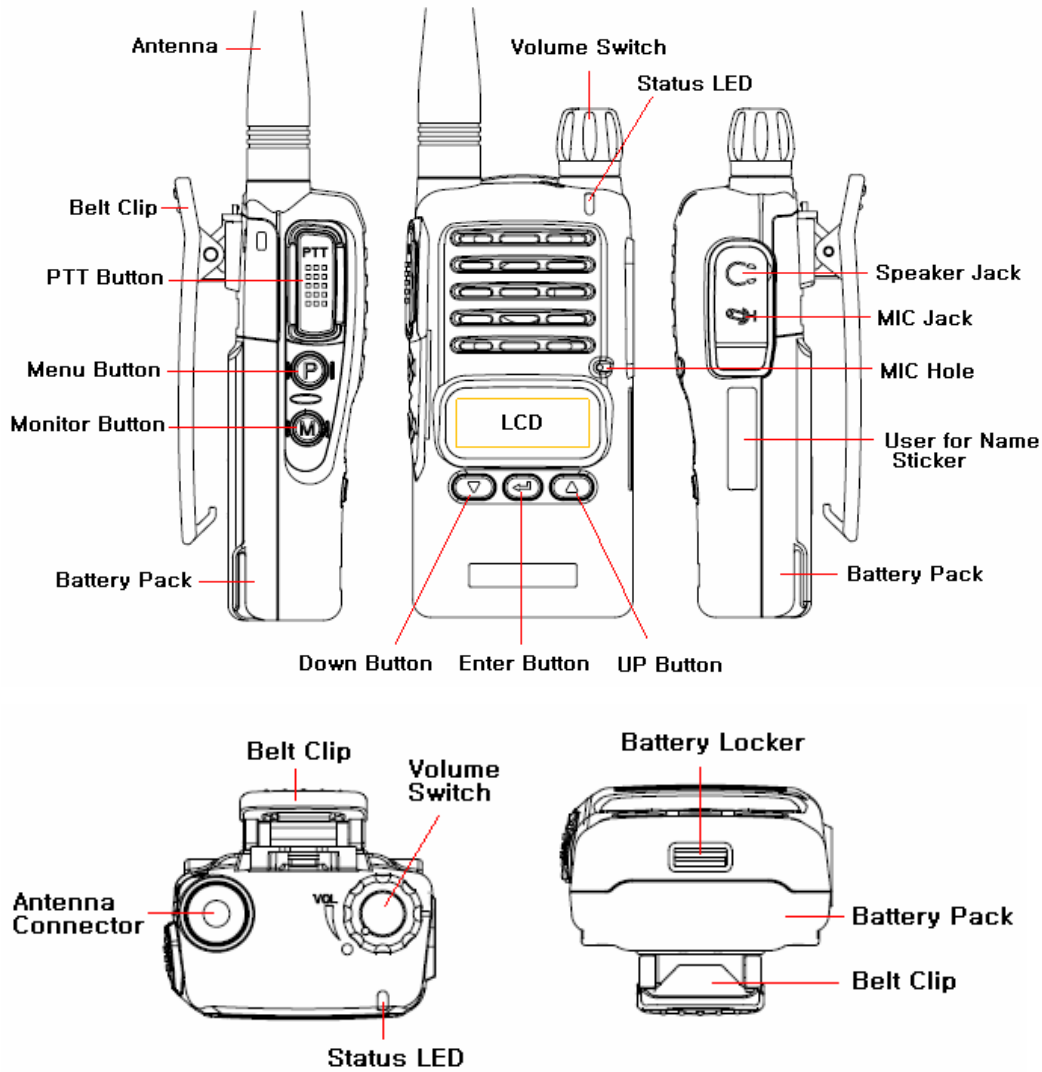
Figure 3-1) Appearance of XV/XU-100 Series Radio
