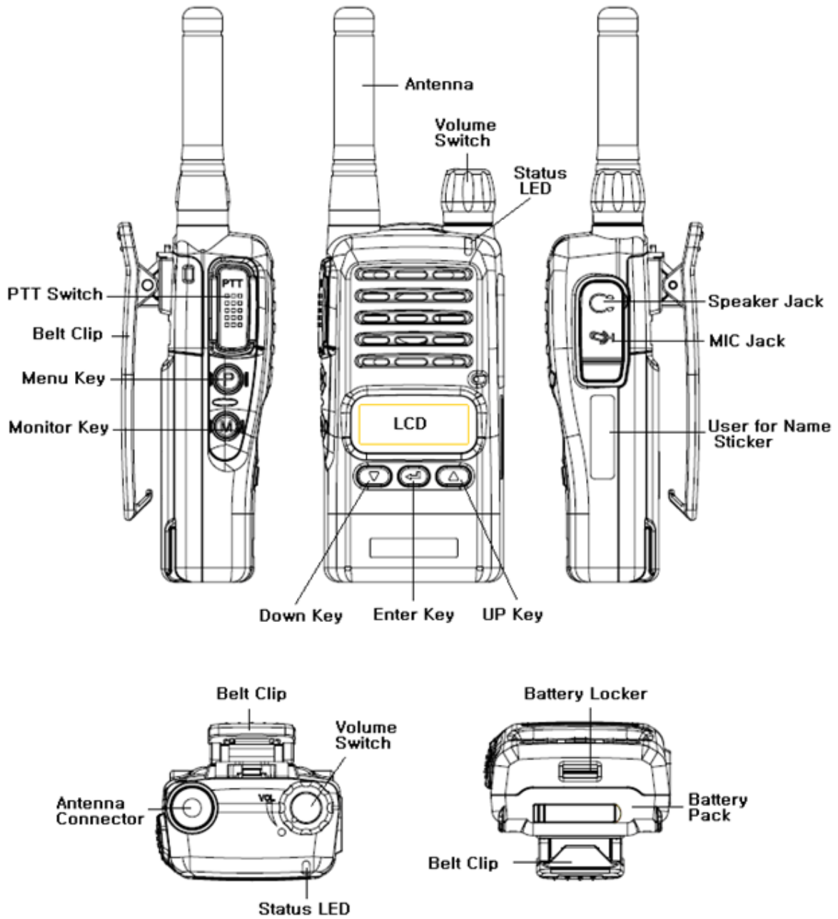
Figure 3-1) Appearance of XV/XU-100 Series Radio
