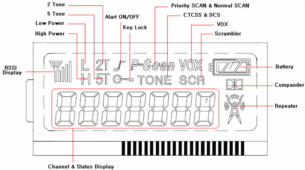
Figure 3-2) XV/XU-100 Series LCD Indication
