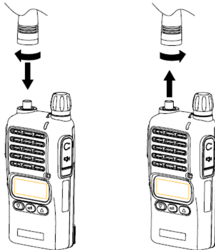
Figure 4-1) Installation and Removing the Antenna
