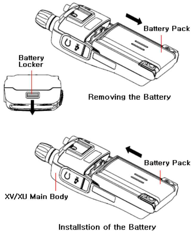
Figure 4-2) Installation and Removing the Battery
