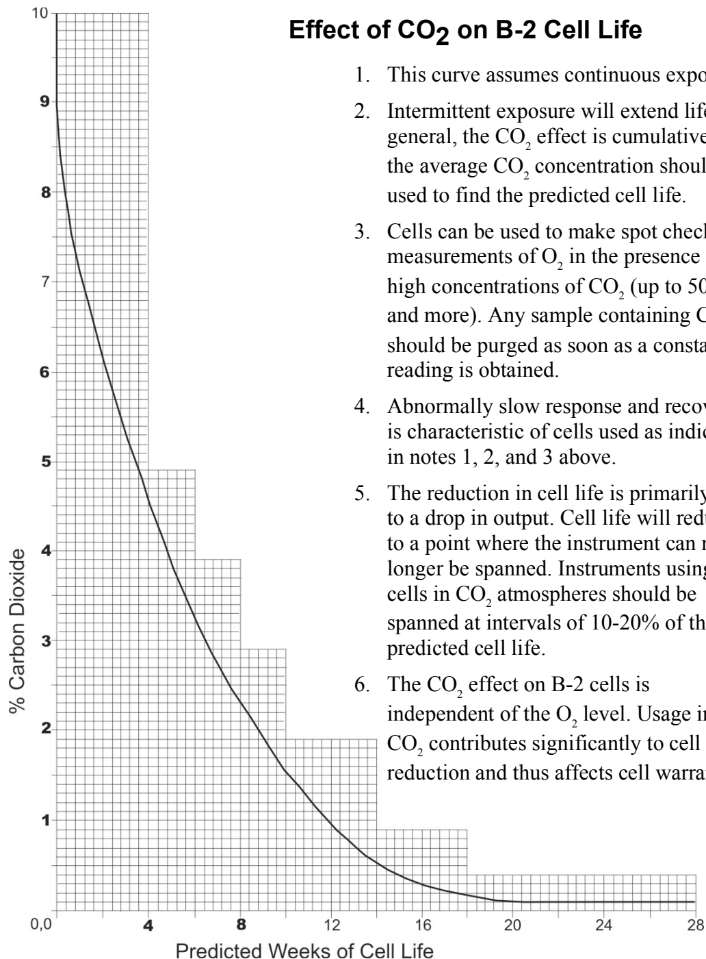
Figure 4-2: Effects of CO 2 on B-2 Cell Life
