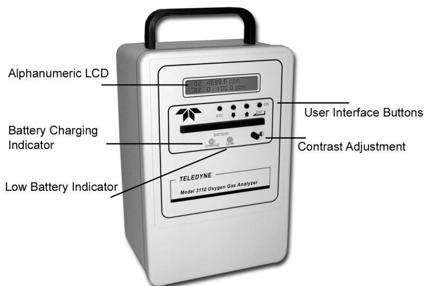
Figure 1-1: Model 3110 Portable Trace Oxygen Analyzer
