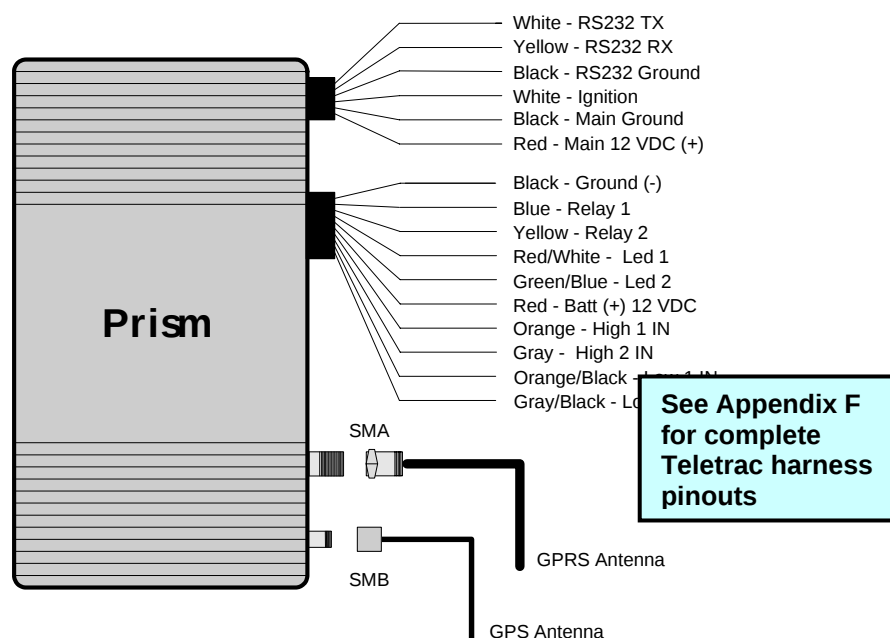
Figure 2 PRISM TM2 Wiring Scheme
