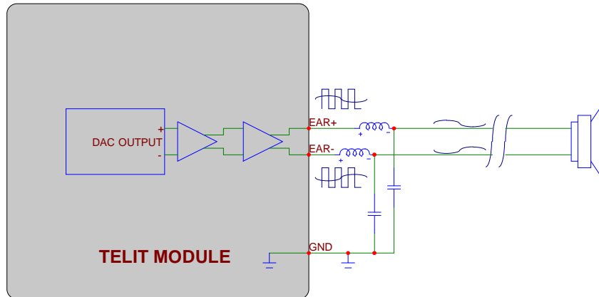
L-C filtering for LOW impedance load.
