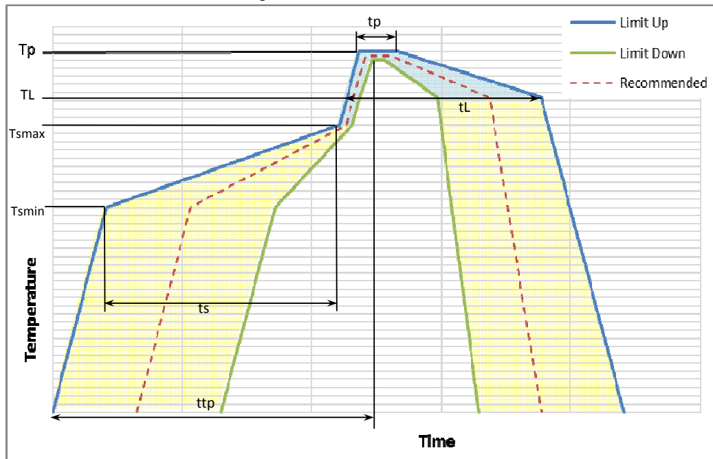
Recommended solder reflow profile
