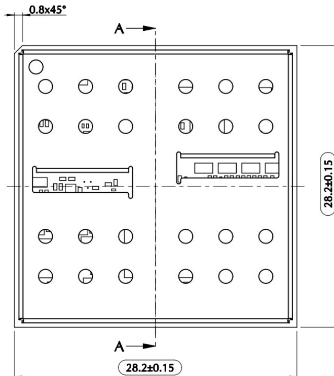
Figure 233: LE910Cx-SV/LA Mechanical Dimensions (Top view)
