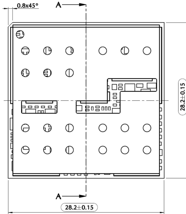
Figure 233: LE910Cx-SV/LA Mechanical Dimensions (Top view)
