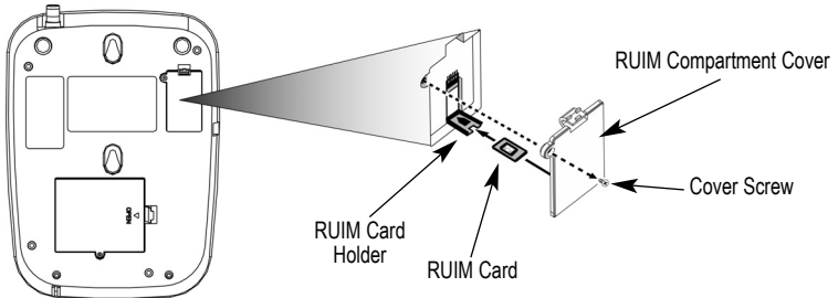
Figure 1 - RUIM compartment cover.
