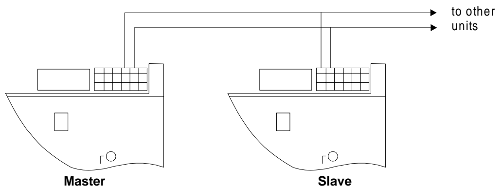
Figure 13: Carrier Phase Synchronisation Interface Connection
