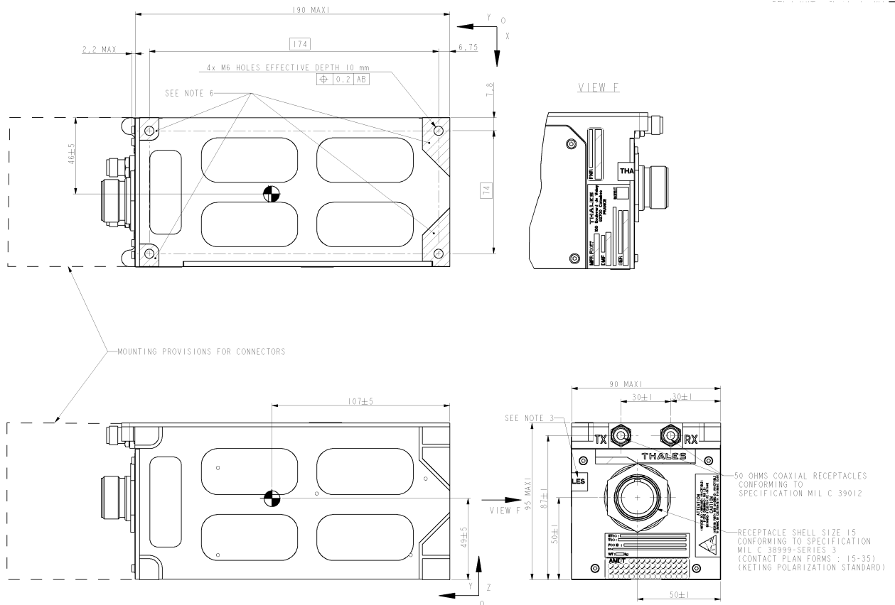
Figure 103 – OVERALL DIMENSIONS
