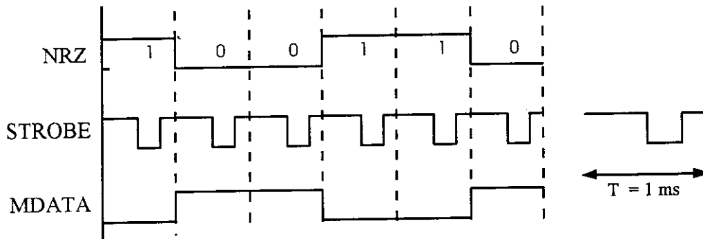
Figure 5-1: Signal timing for the ISO2 interface. Period for NRZ data is roughly 1 ms
