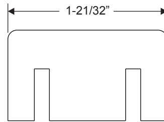
Steel RPER30C (3/0) RPER36C (3/6)
