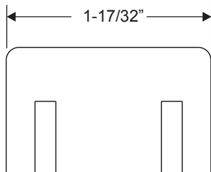
Fiber-Classic/Smooth-Star RPSSF CER30C
