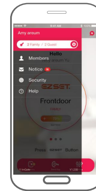
Touch "NOTICE"
