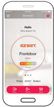
Touch "History"
