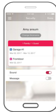
Nickname change
