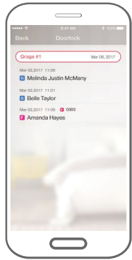
Open history
