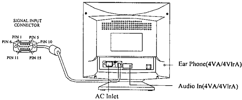
Figure 2 Connecting Cables
