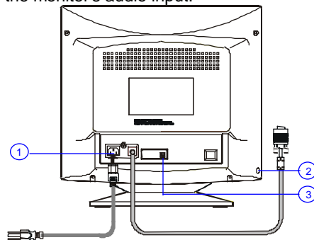
Figure 2 Connecting Cables
