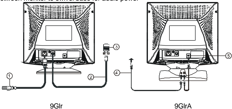
Figure 2 Connecting Cables
