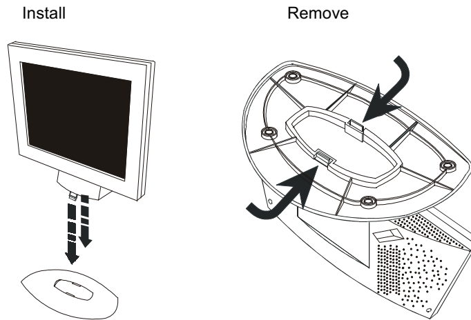
Figure 1 Installing and Removing the Swivel Base
