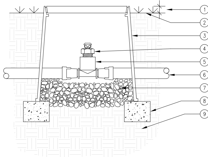
SECTION/ELEVATION
