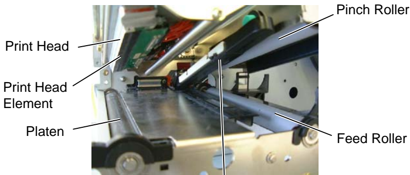
Black Mark Sensor/ Feed Gap Sensor
