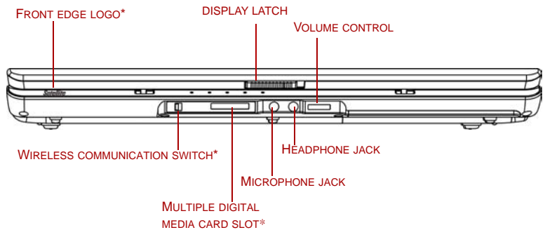
Figure 2-1 Front of the computer with display closed
