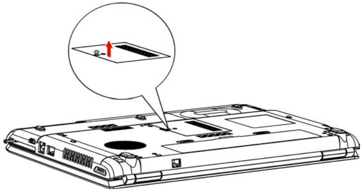
Figure 8-5 Removing the cover
