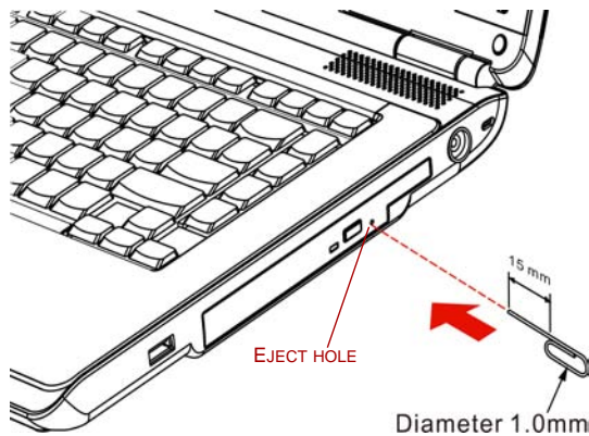
Figure 4-3 Manual release with the eject hole
