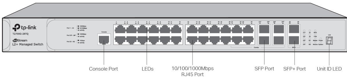
Figure 2-1 Front Panel
