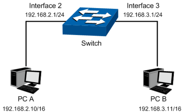
Figure 10-21 ARP Application
