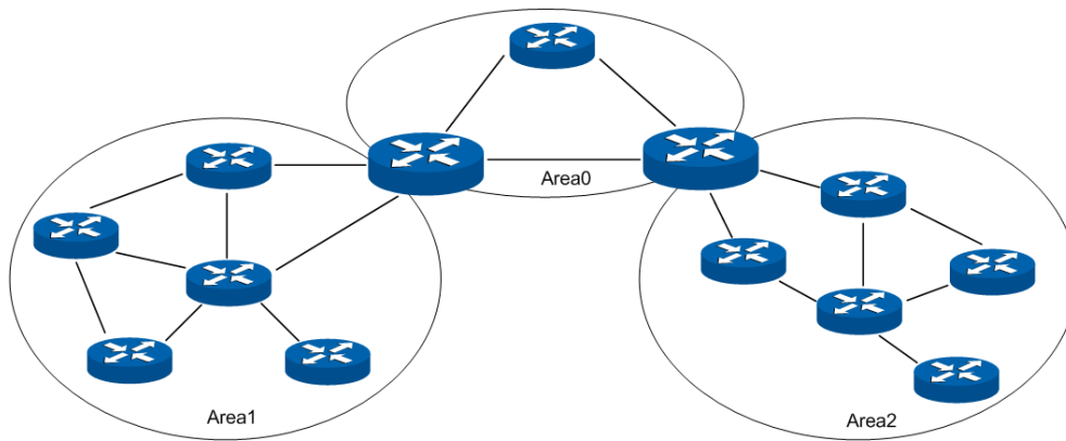
Figure 10-34 Area Model
