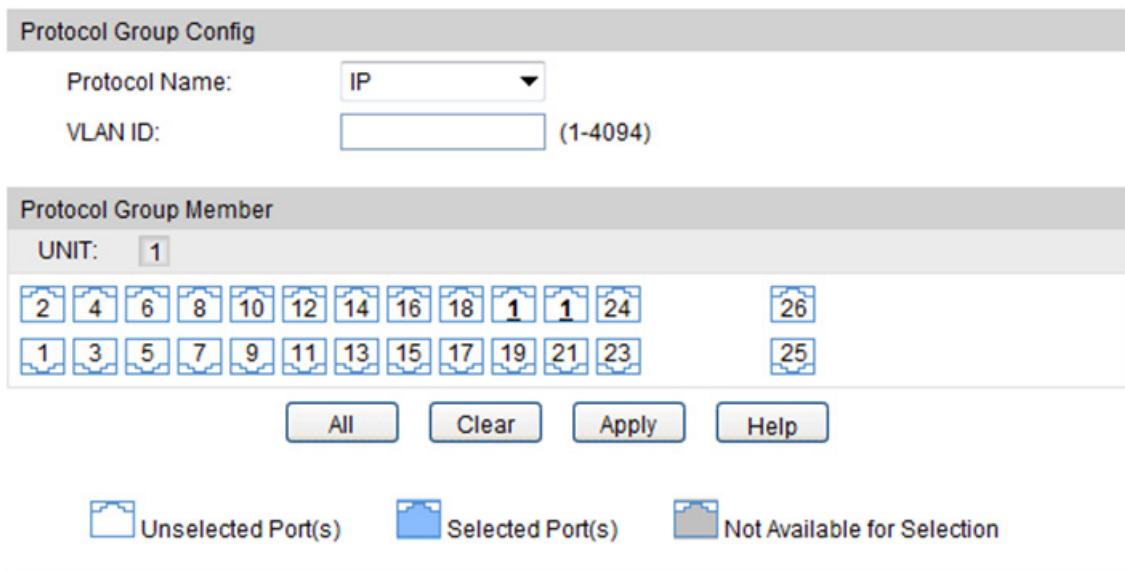
Figure 7-10 Enable Protocol VLAN for Port
