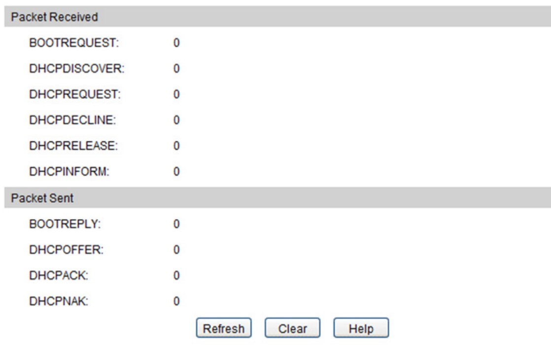
Figure10-15 Statistics
