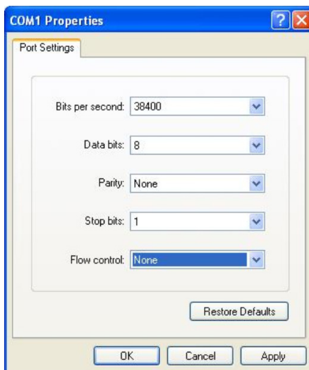
Figure 19-5 Port Settings
