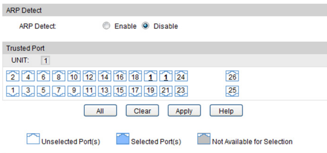
Figure 14-14 ARP Detect
