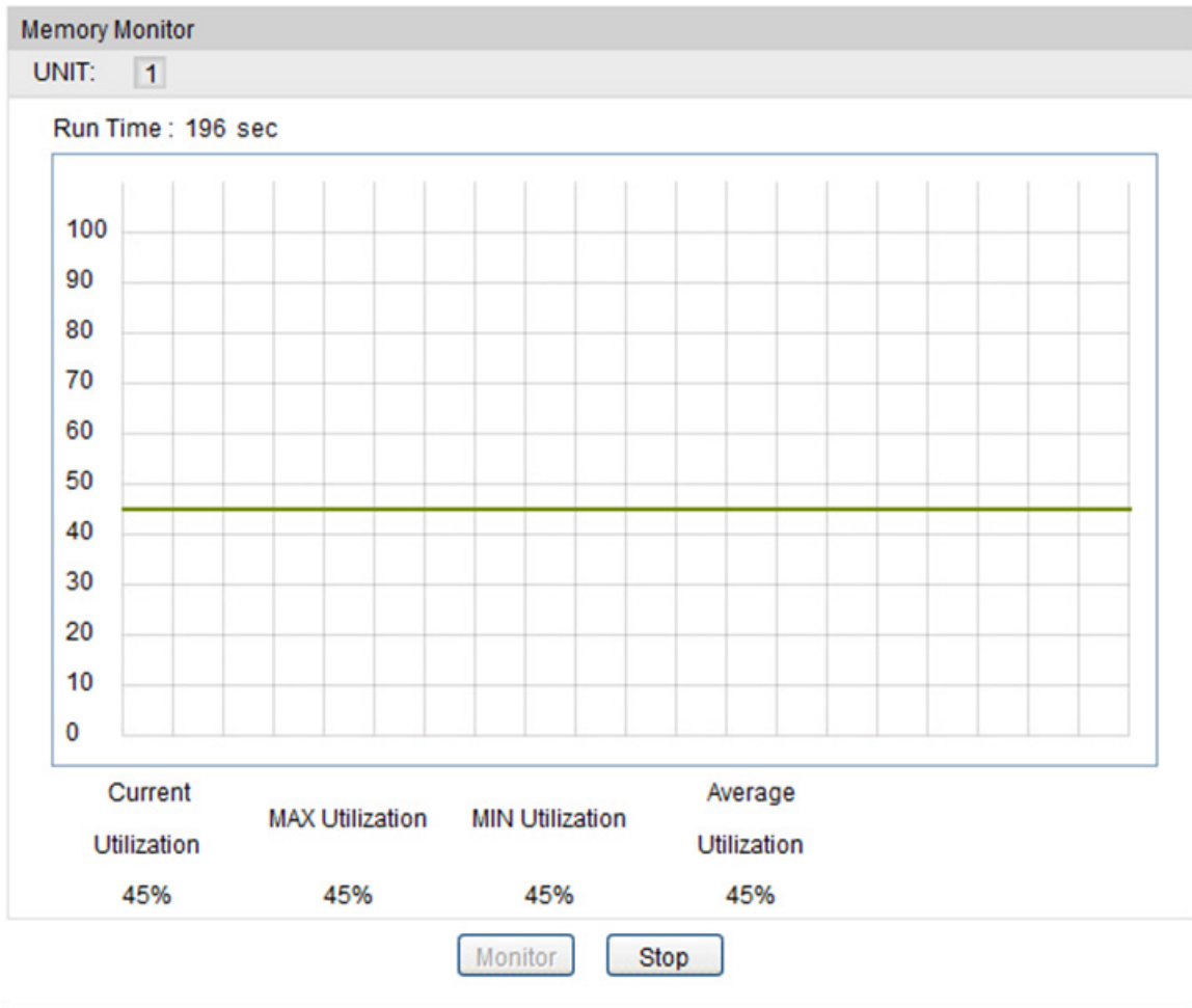
Figure18-2 Memory Monitor
