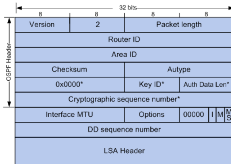
Figure 10-41 DD Packet
