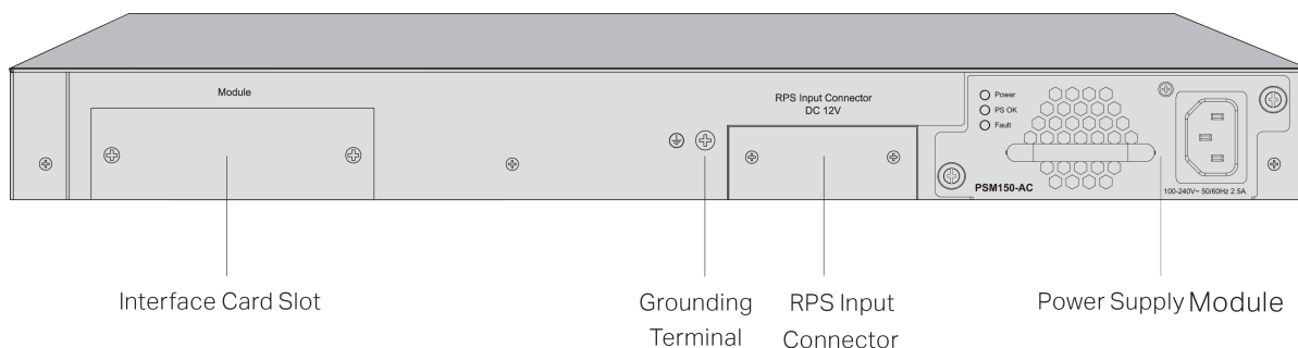
Figure 2-2 Rear Panel (1)
