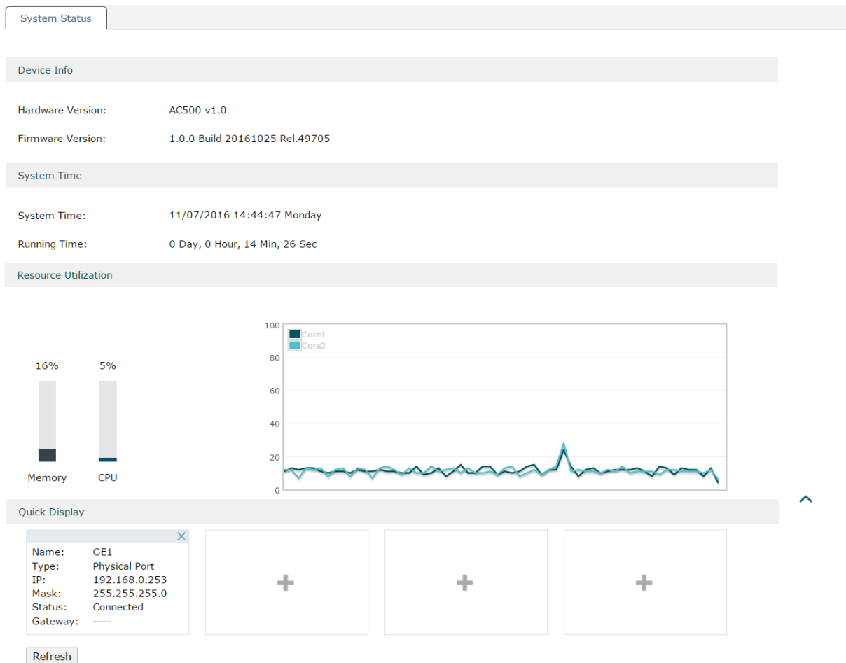
Figure 2-1 System Status
