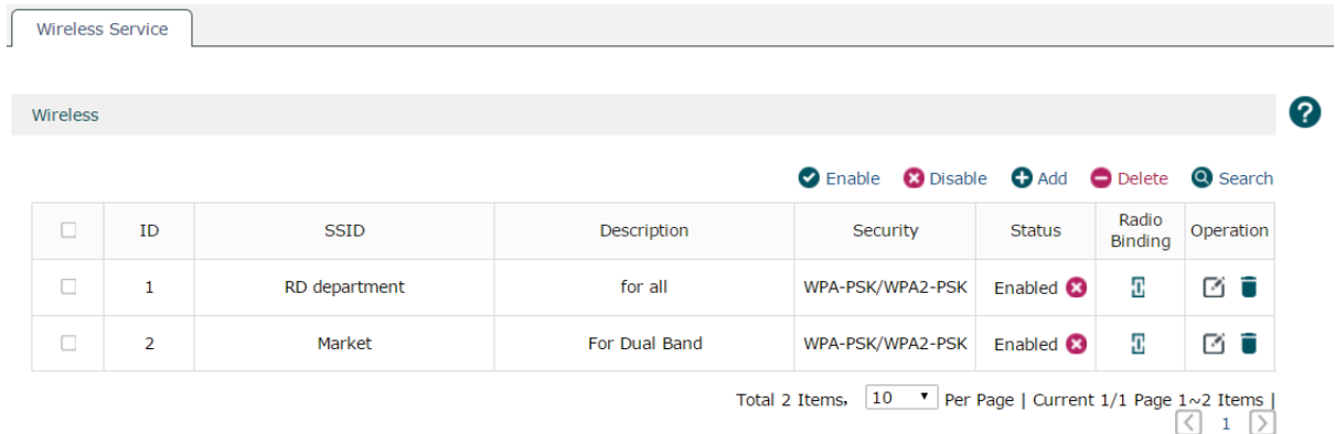
Figure 6-1 Wireless Service
