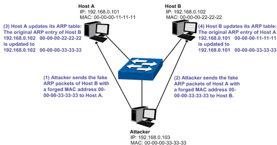
Figure 14-18 Man-In-The-Middle Attack
