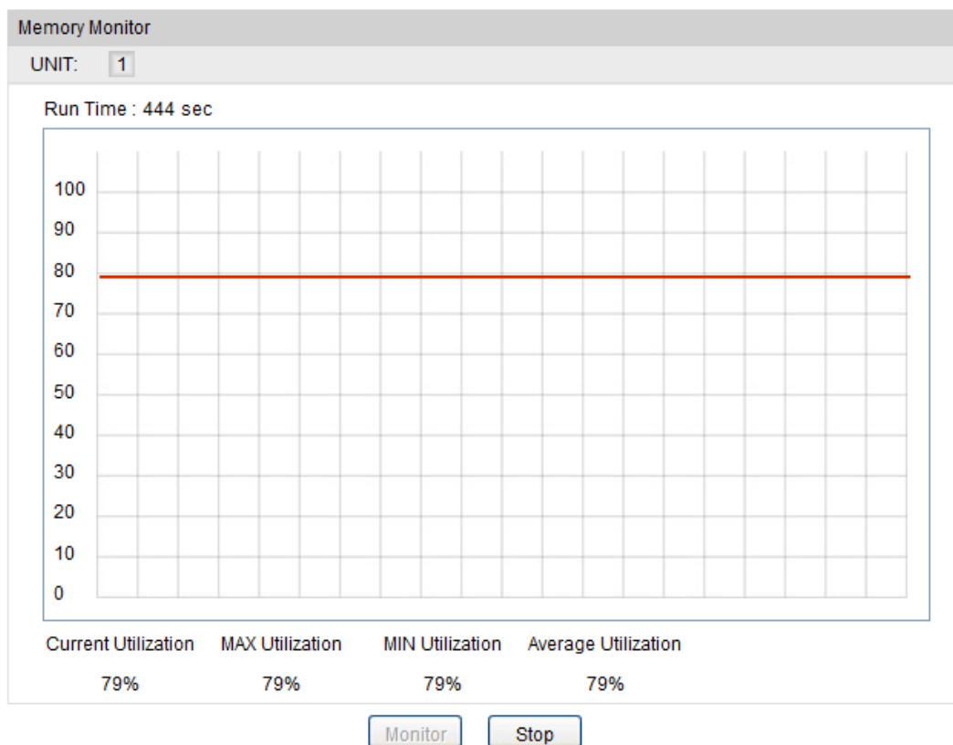
Figure 17-2 Memory Monitor
