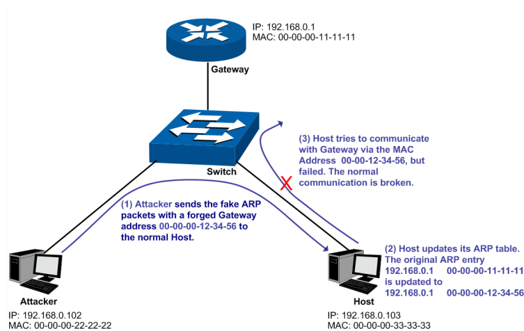
Figure 14-15 ARP Attack - Imitating Gateway
