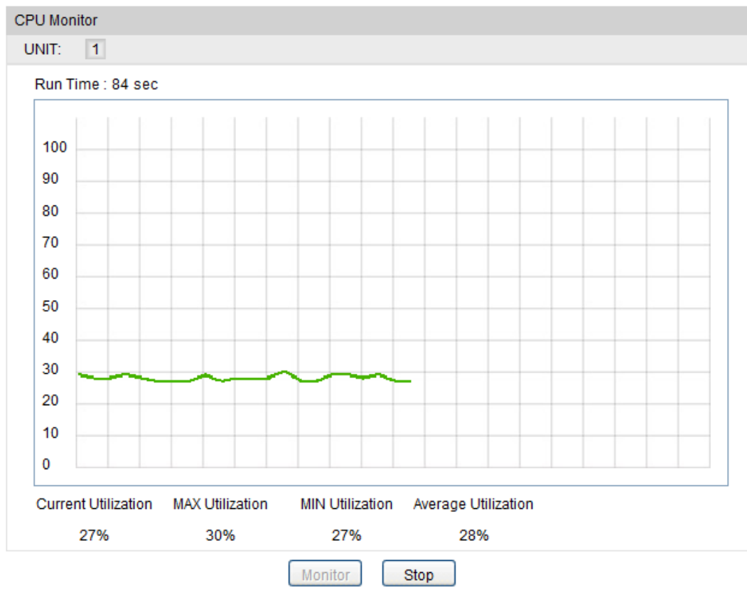
Figure 17-1 CPU Monitor
