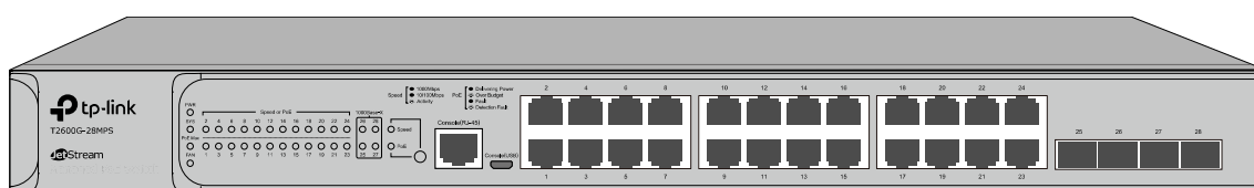
Figure 2-3 Front Panel of T2600G-28MPS
