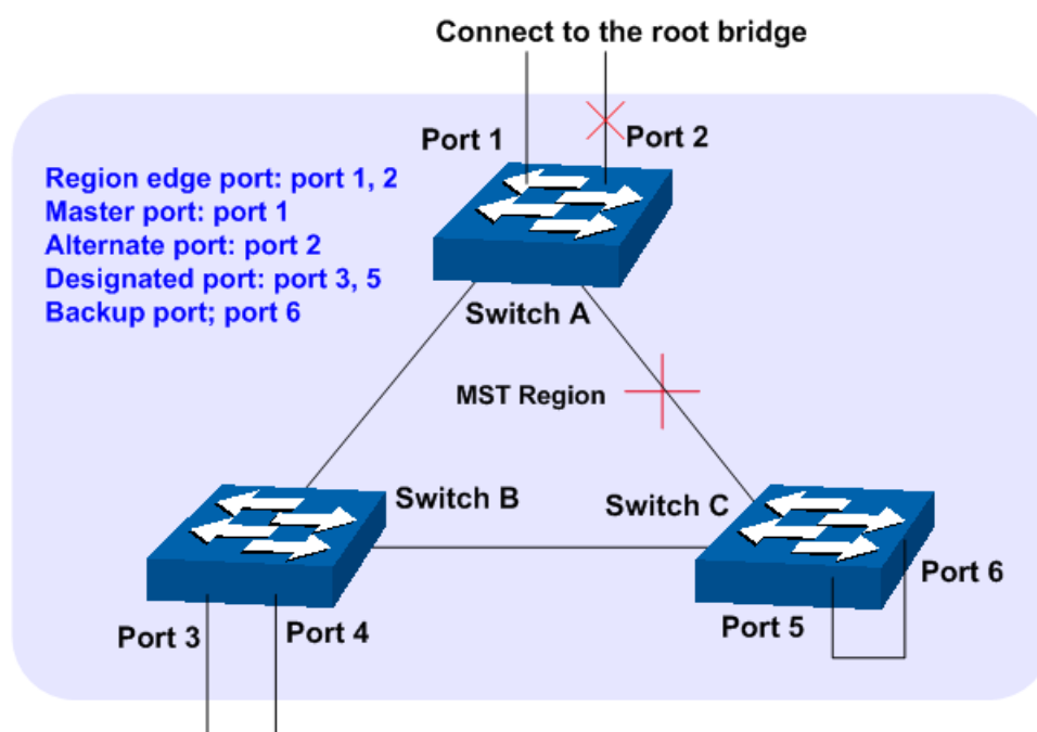
Figure 7-3 Port roles
