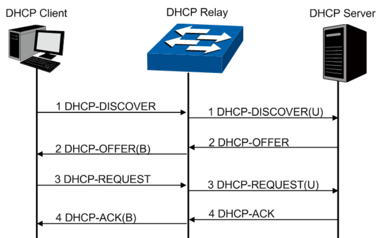
Figure 10-22 DHCP Relay Process
