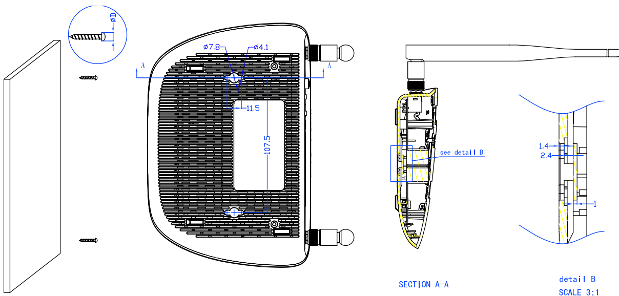
Figure 2-1 Wall-mount Install
