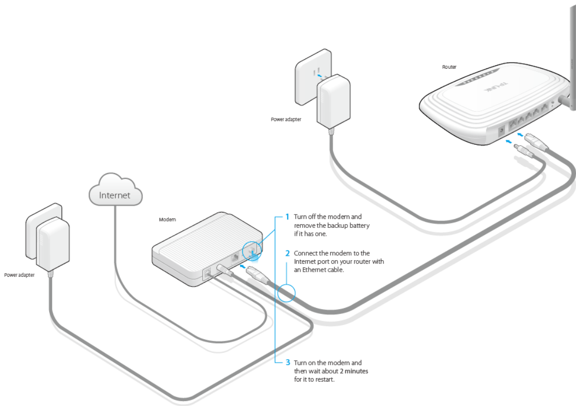
Figure 2-1 Hardware Installation
