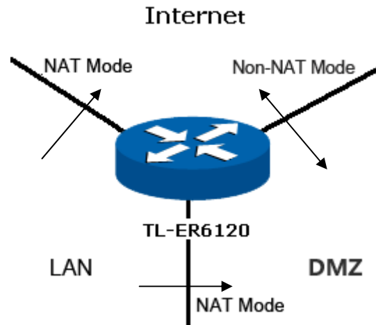
Figure 3-16 DMZ – Public Mode
