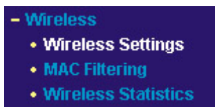
Figure 5-9: Wireless menu
