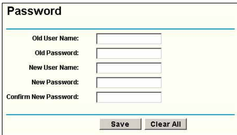
Figure 5-43: Password
