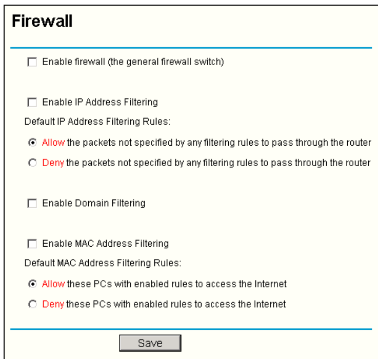
Figure 5-24: Firewall Settings
