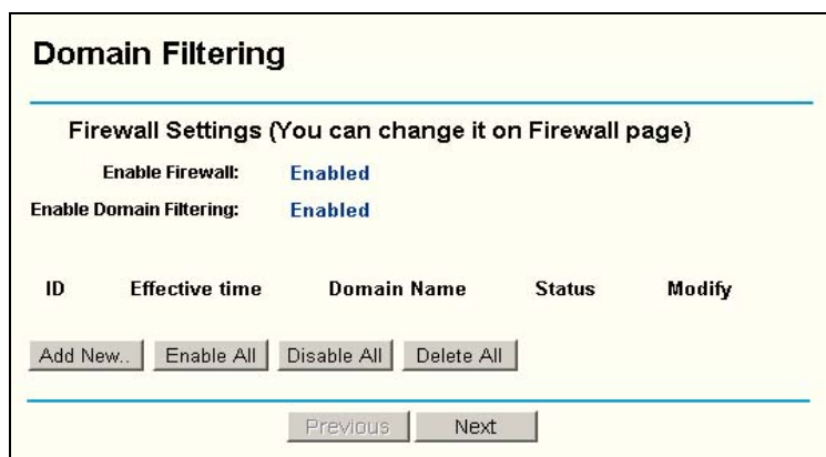
Figure 5-27: Domain Filtering
