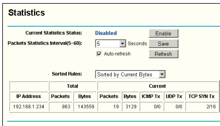
Figure 5-45: Statistics
