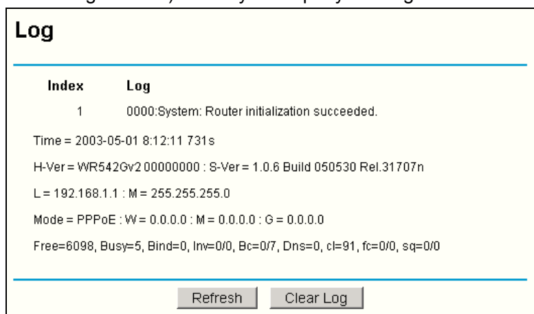
Figure 5-44 System Log
