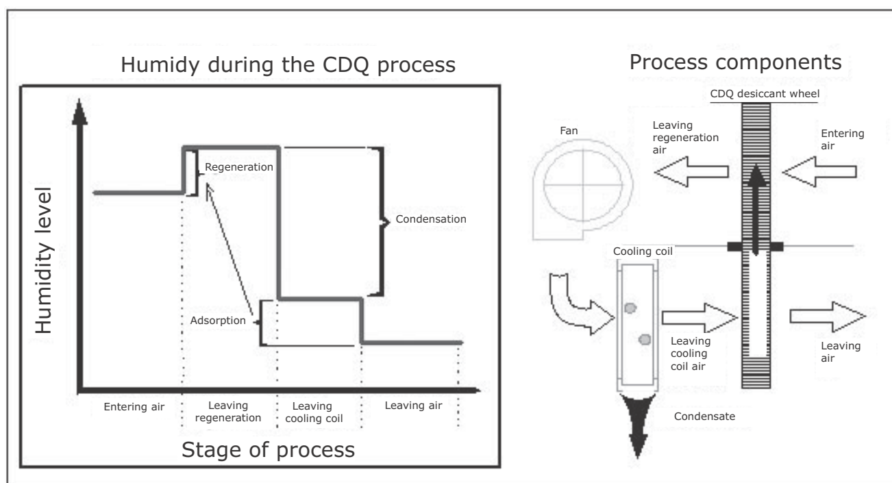
Figure 24. Dehumidification with CDQ (Cool, Dry, Quiet) desiccant dehumidification units
