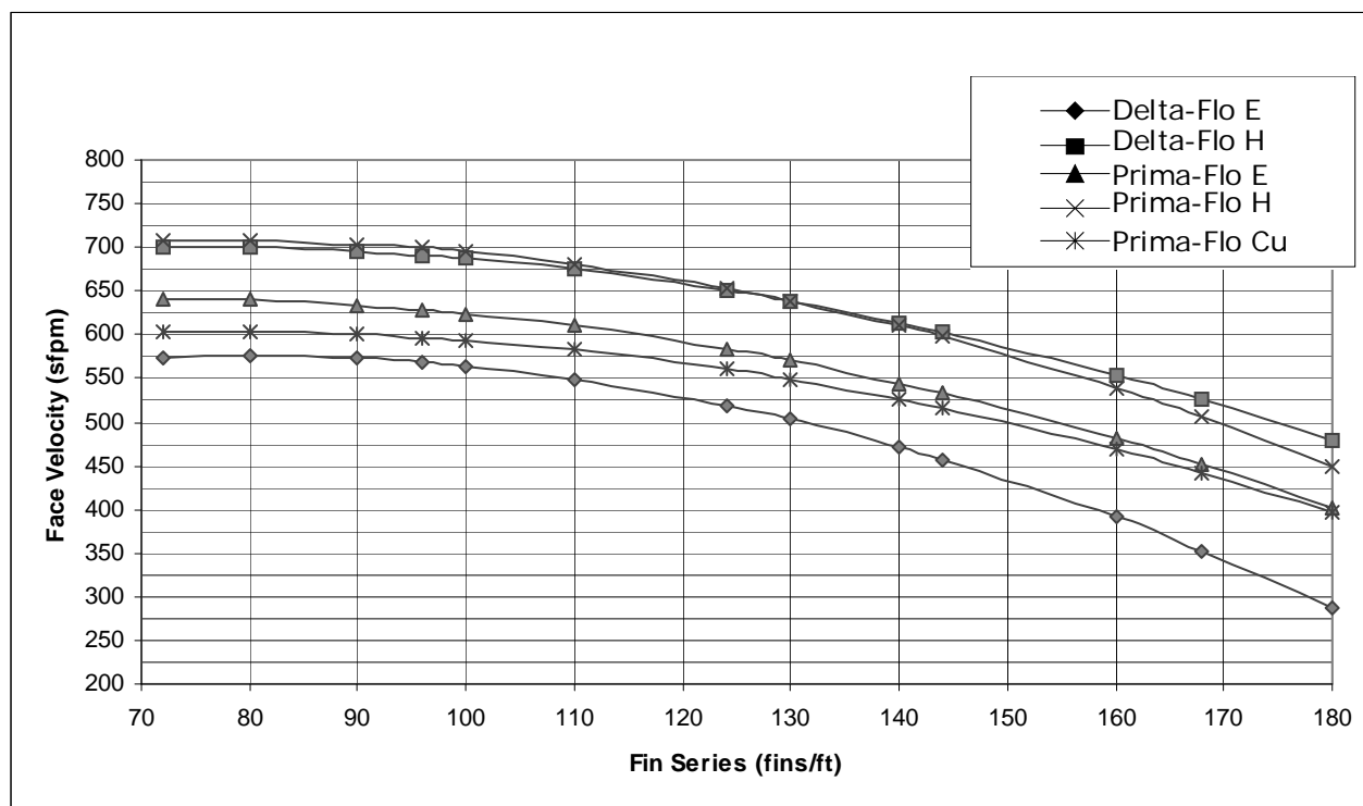
Figure 69. Face velocity limits for moisture carryover with uncoated coils in unit sizes 35 and 40
