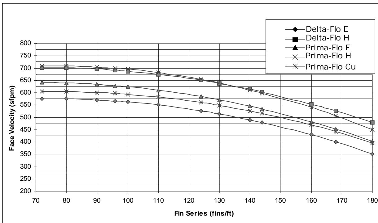
Figure 69. Face velocity limits for moisture carryover with uncoated coils in unit sizes 35 and 40
