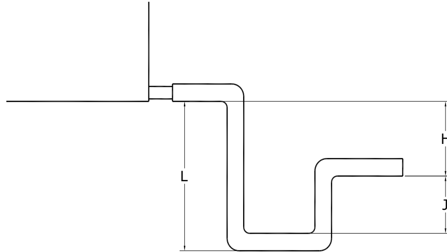
Figure 17. Drain pan trapping for positive and negative pressure applications
