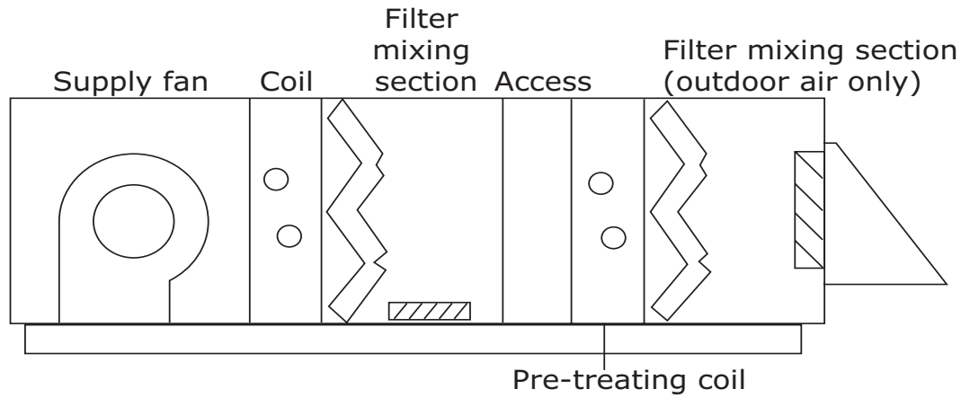
Figure 27. Outdoor air pre-treating split dehumidification unit
