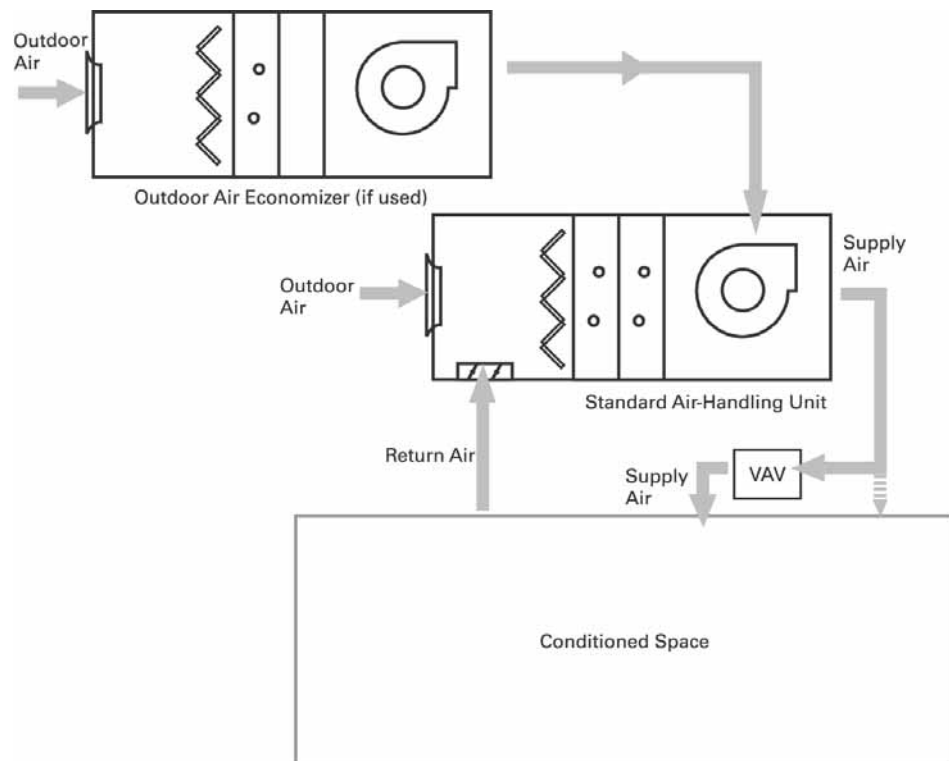
Figure 20. Dual-path design
