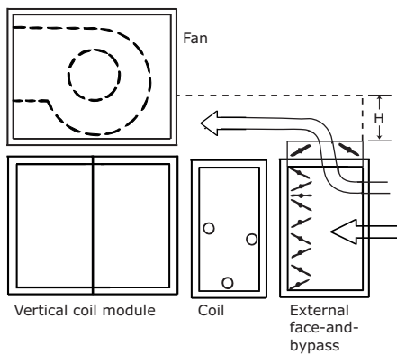
Figure 47. Configuration C
