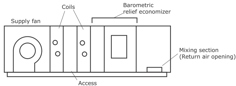
Figure 23. Building pressurization with a barometric relief economizer arrangement
