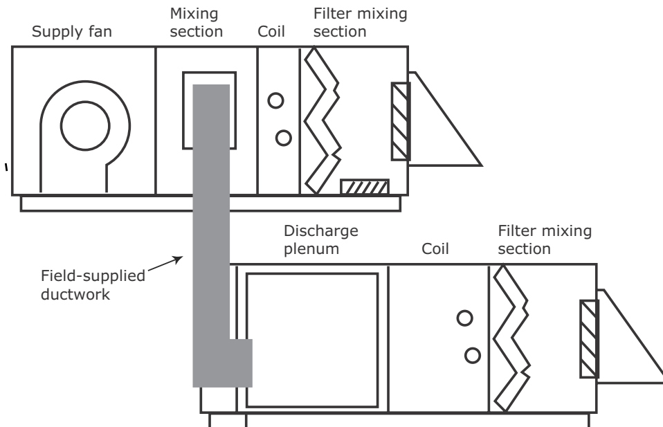
Figure 28. Split dehumidification with outdoor units
