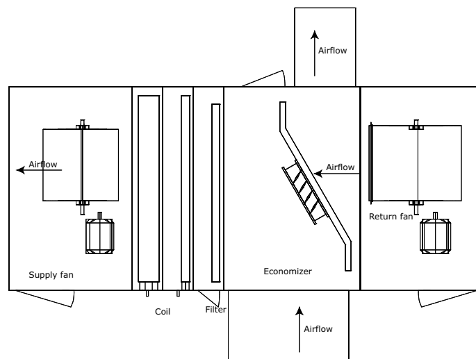
Figure 21. Return fan and economizer arrangement for outdoor units
