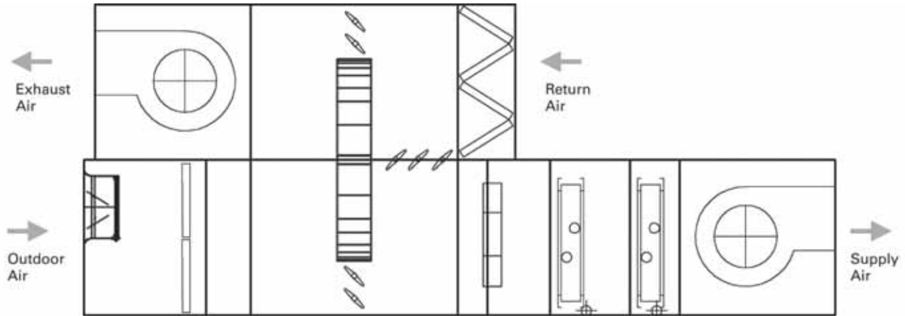
Figure 29. Energy-recovery with a total energy wheel in indoor unit
