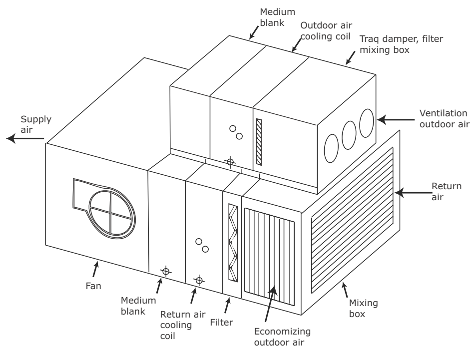
Figure 26. Horizontal split dehumidification indoor unit (SDU)
