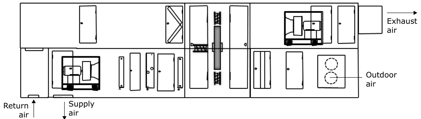
Figure 30. Energy-recovery with a total energy wheel in outdoor unit
