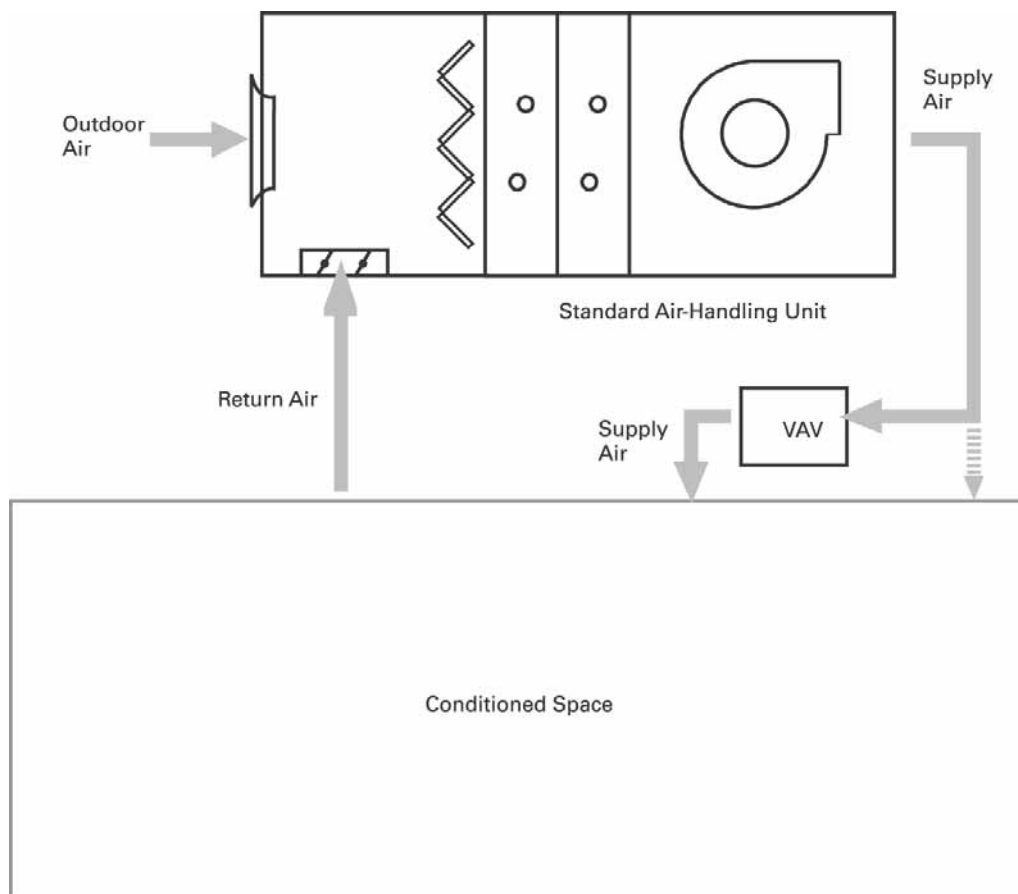
Figure 19. Single-path design
