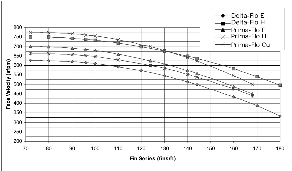
Figure 67. Face velocity limits for moisture carryover with uncoated coils in unit sizes 14 to 17
