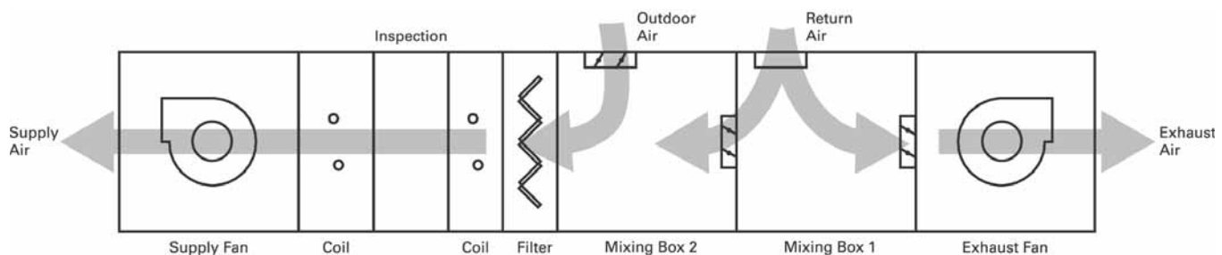
Figure 22. Exhaust fan and economizer arrangement
