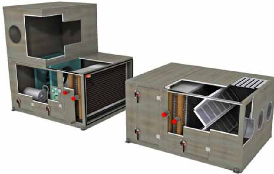
Figure 1. Trane Performance Climate Changer™ air handler
