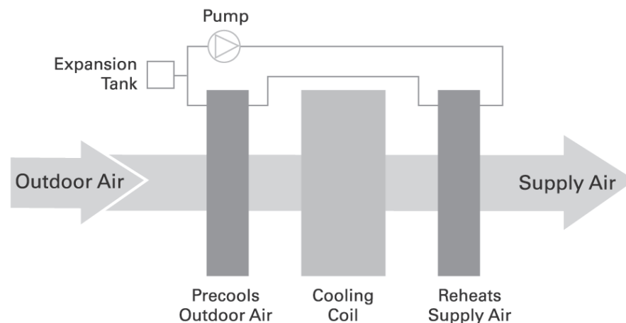
Figure 25. Series dehumidification with coil run-around loops
