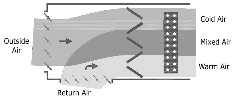
Figure 12. Protect coils from freezing by addressing air stratification
