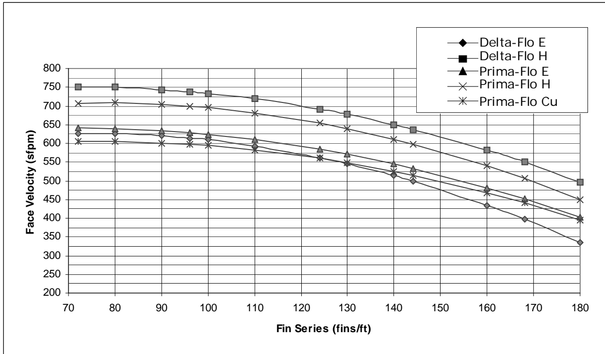
Figure 71. Face velocity limits for moisture carryover with uncoated coils in unit size 66
