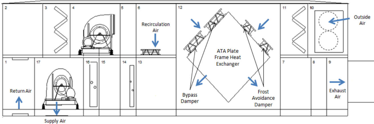
Figure 32. Energy recovery with air-to-air plate from heat exchanger
