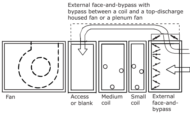
Figure 46. Configuration B
