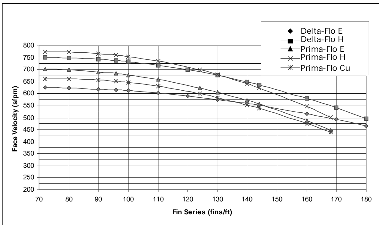
Figure 65. Face-velocity limits for moisture carryover with uncoated coils in unit sizes 3 to 10
