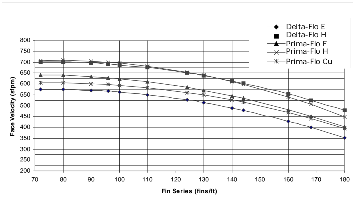
Figure 72. Face velocity limits for moisture carryover with uncoated coils in unit sizes 80 to 120
