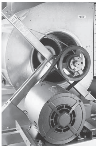
Figure 55. Trane offers a wide variety of fan choices
