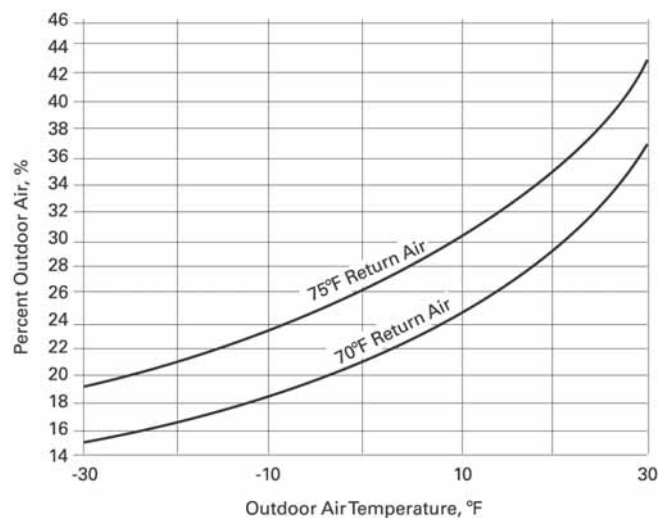
Figure 36. Blender performance with 55°F leaving air temperature
