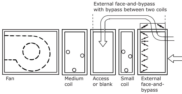
Figure 45. Configuration A
