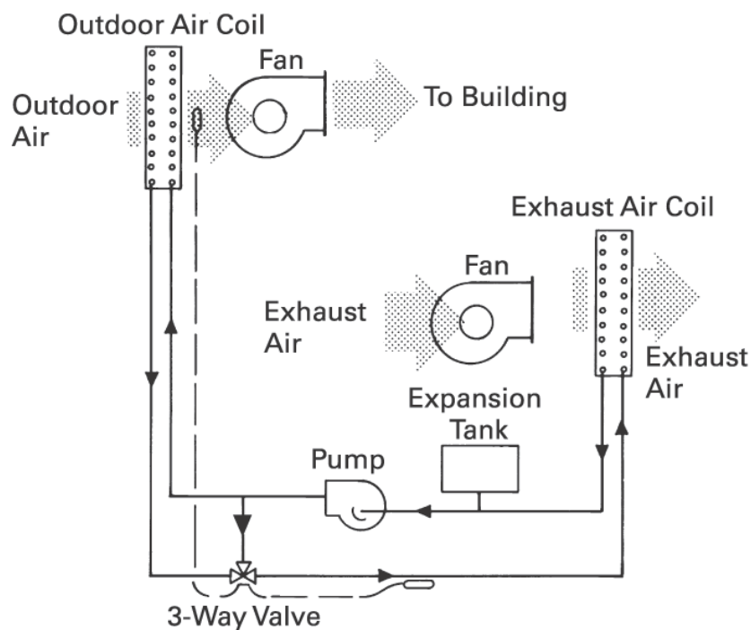
Figure 31. Energy recovery with a runaround coil loop
