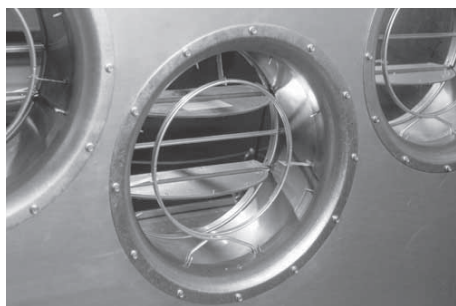
Figure 48. Traq dampers measure and control ventilation airflow.
