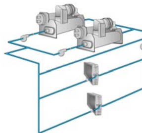
primary-secondary system
