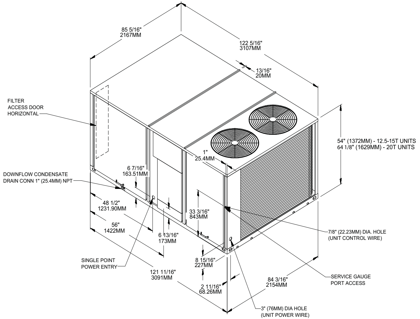
Figure 2. Heat pump models - 12½ - 20 tons
