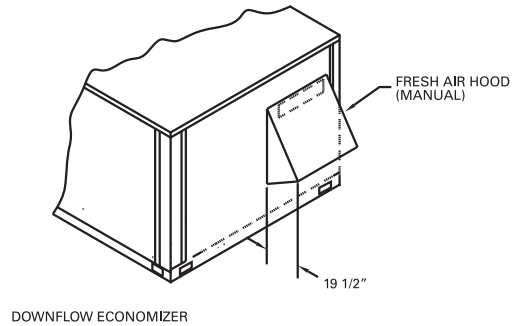
Figure 9. Fresh air hood (downflow units)
