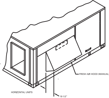
Figure 8. Fresh air hood (horizontal units)
