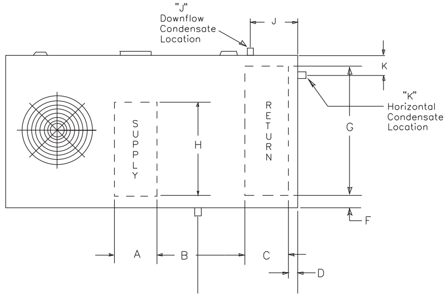
Figure 7. Downflow & horizontal condensate locations
