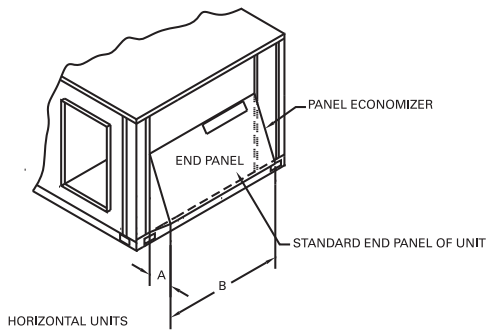
Figure 12. Economizer - horizontal units
