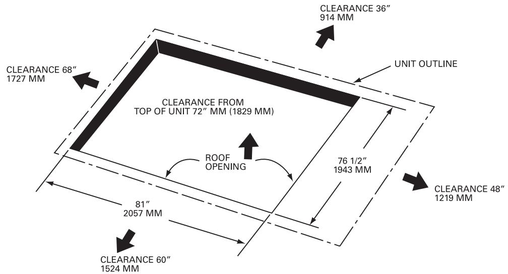
Figure 6. Heat pump models - 12½ - 20 tons
