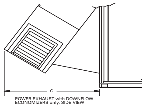
Figure 11. Power exhaust - downflow economizers - side view
