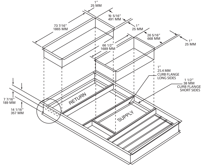
Figure 5. Heat pump models - 12½ - 20 tons
