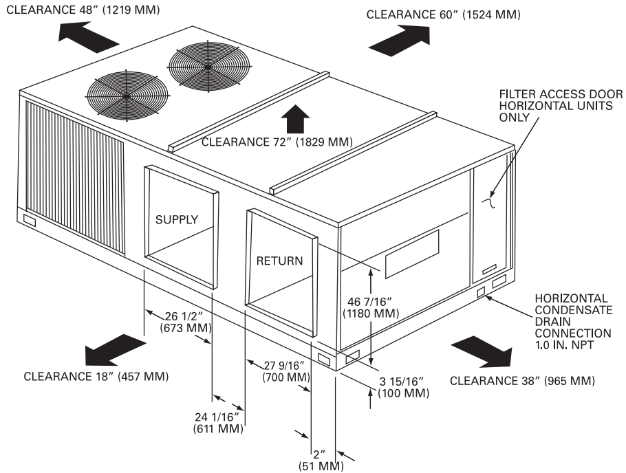
Figure 3. Heat pump models - 12½ - 20 tons
