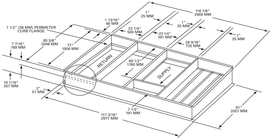
Figure 4. Heat pump models - 12½ - 20 tons
