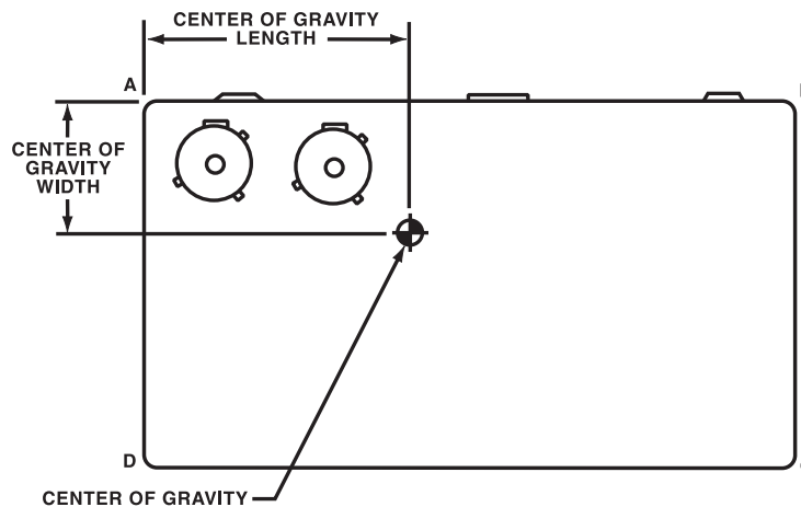
Figure 14. Center of gravity
