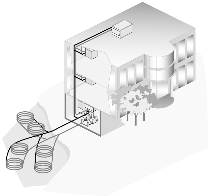
Figure 6: Ground source surface water system
