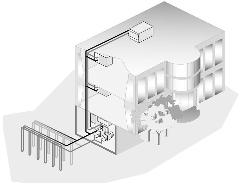
Figure 5: Ground source geothermal system
