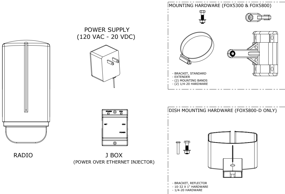
Figure 1. Components of TrangoFOX Subscriber Unit
