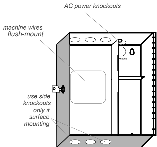
FIGURE 3: Mounting & Knockouts
