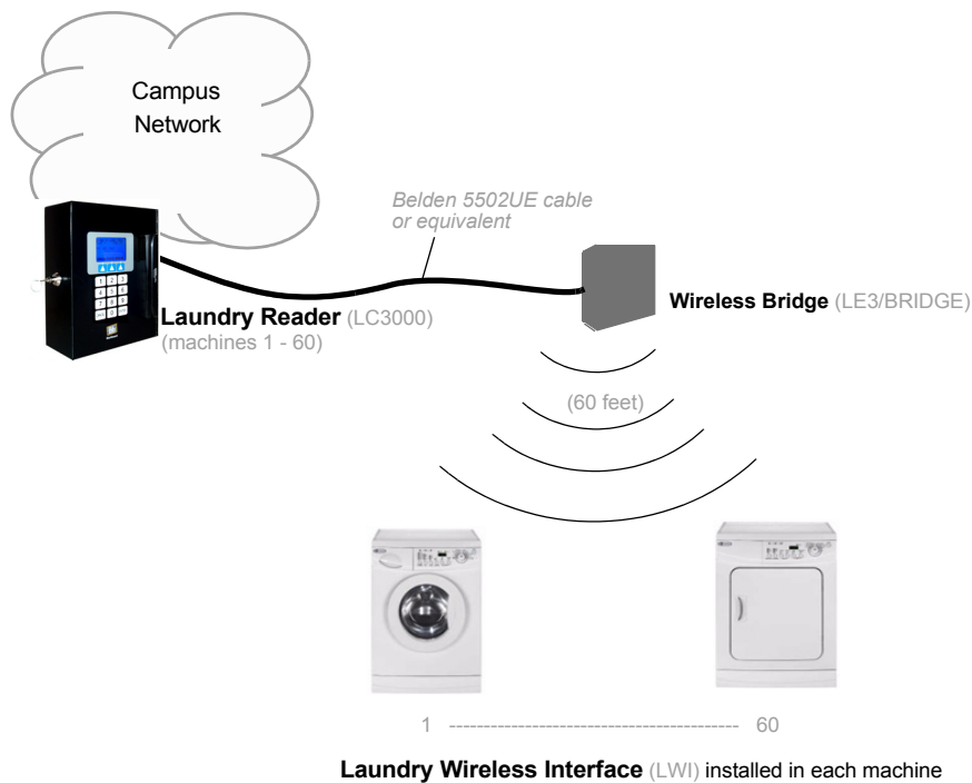
FIGURE 2: Wireless Laundry Center Solution
