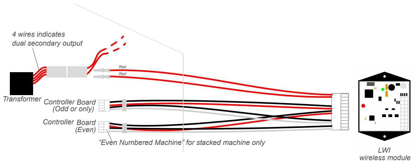
FIGURE 24: LWI3020 installation in Speed Queen/Alliance laundry machine
