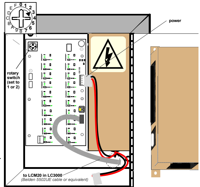
FIGURE 14: LCM20 and LE3/PSENCL Connections
