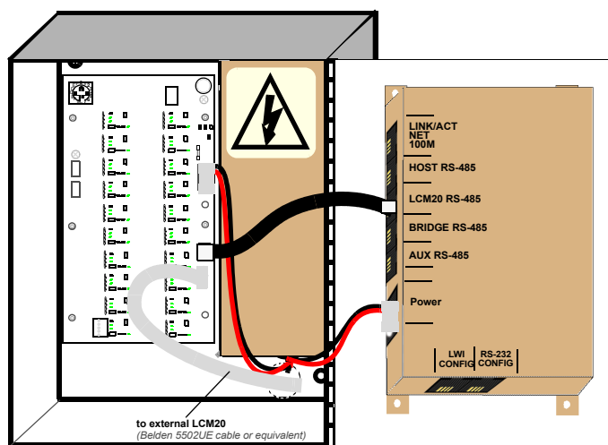
FIGURE 11: LCM20 Connections
