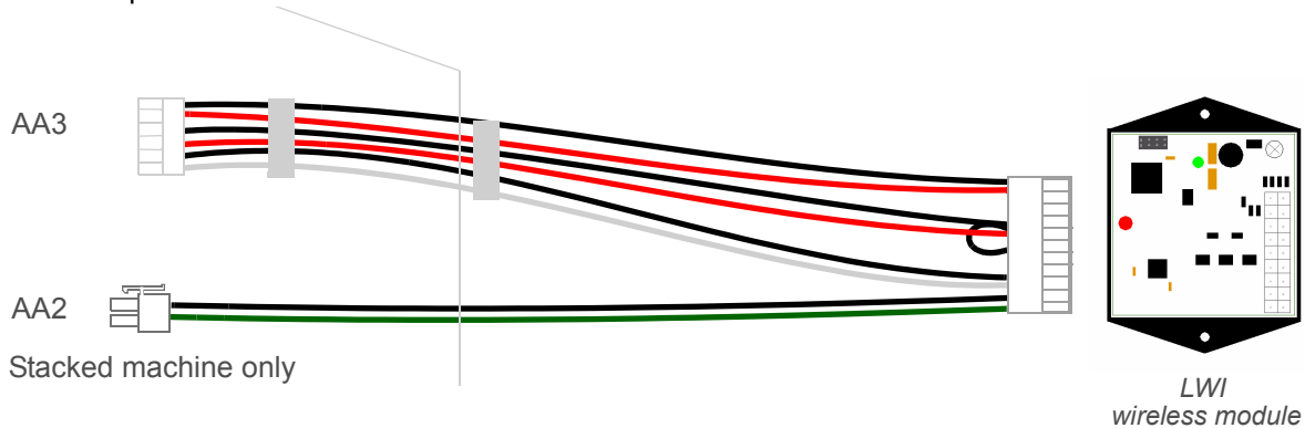
FIGURE 23: LWI3010 installation in Maytag laundry machine
