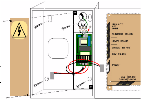
FIGURE 4: Power Installation
