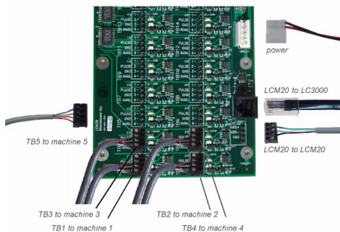
FIGURE 11: LCM20 Connections
