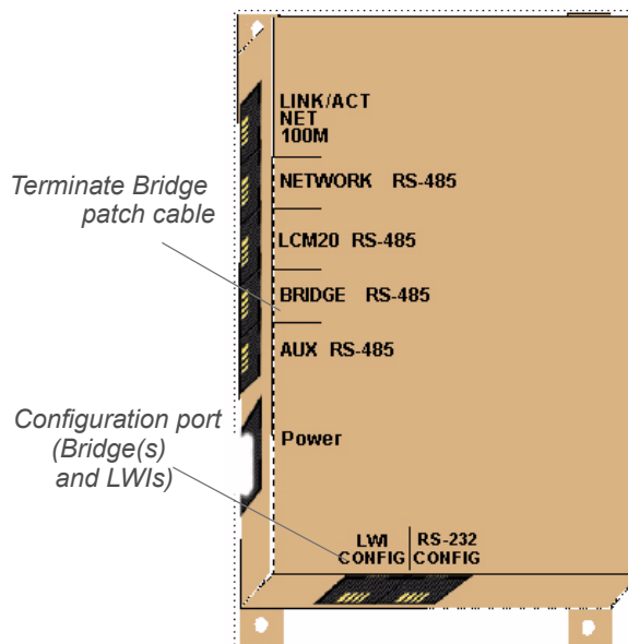
FIGURE 20: Bridge Connections
