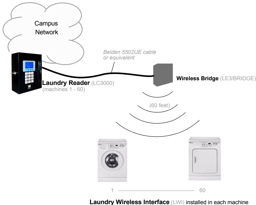
FIGURE 19: Wireless Laundry Center Solution
