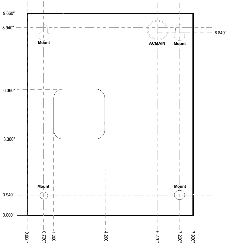
FIGURE 26: LC3000 Dimensions
