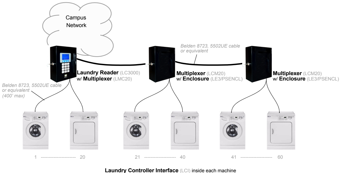
FIGURE 1: Wired LC3000 Laundry Center
