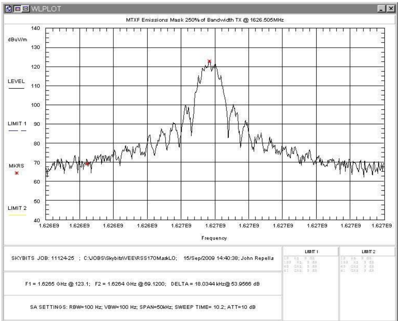
Figure 8: Spectrum Plot, Low Channel @ +/-250% of BW
