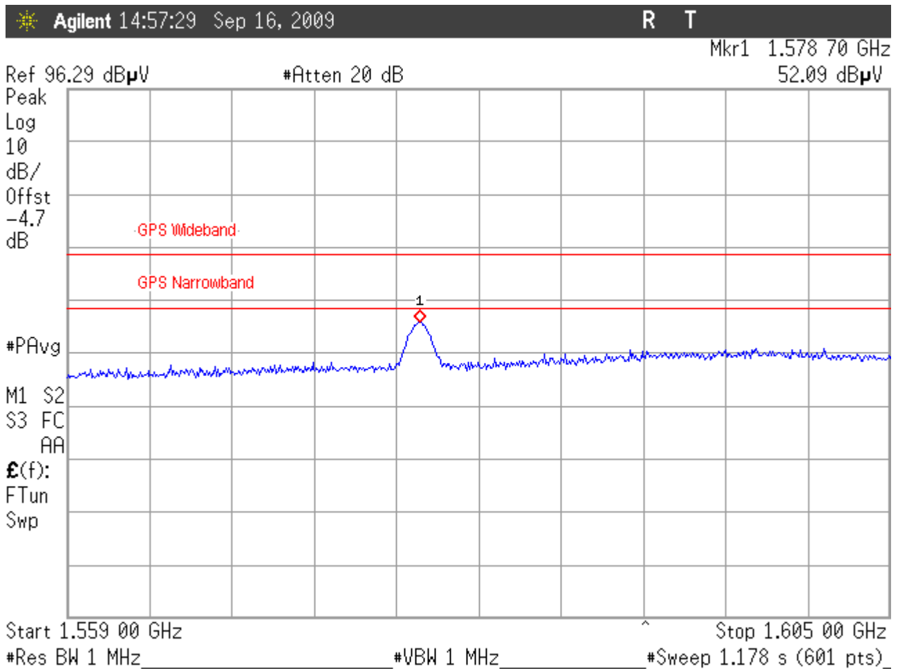
Figure 21: GPS Band Emissions High Channel, 1559 – 1605MHz Horizontal Antenna Polarity
