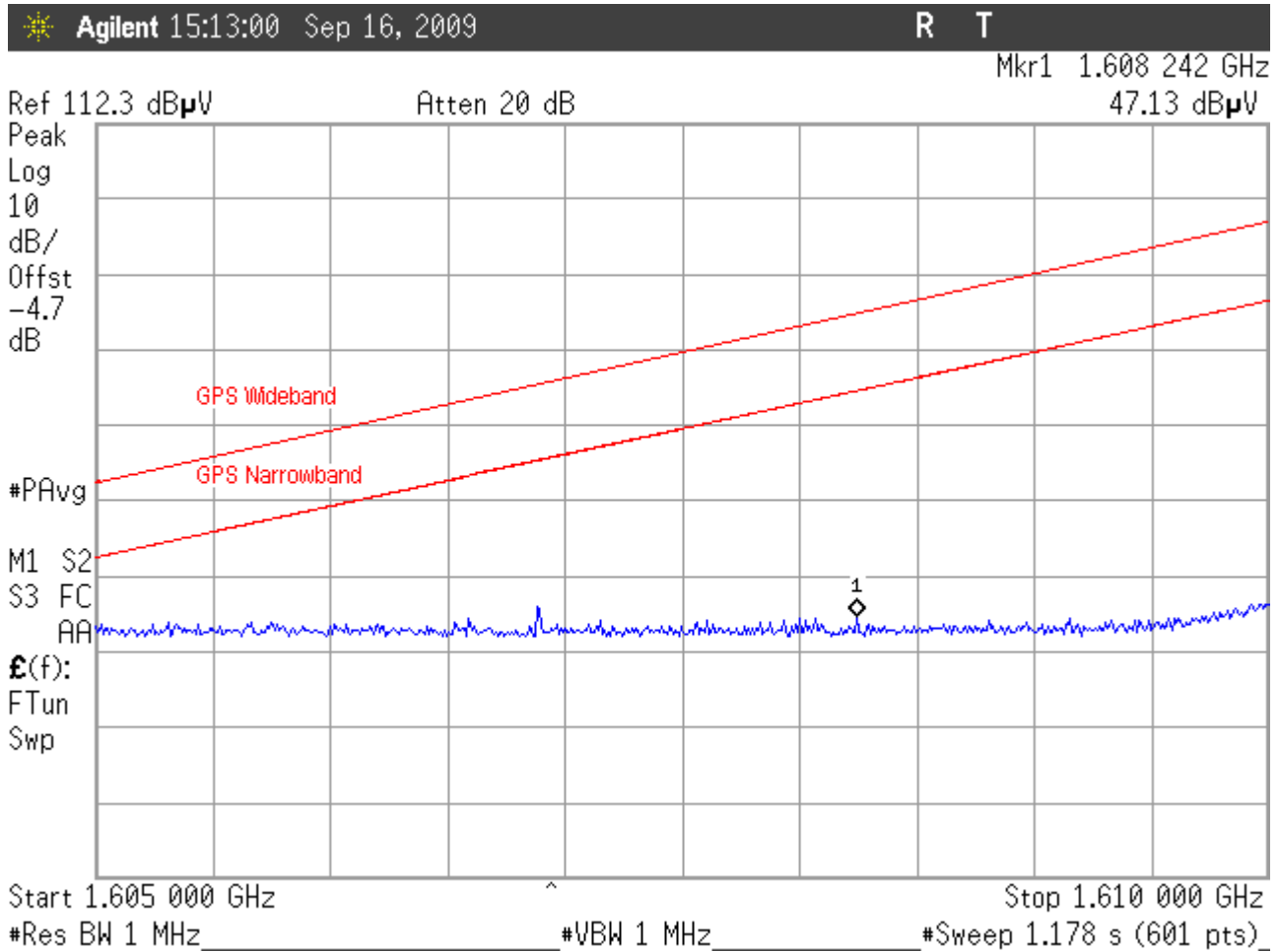
Figure 22: GPS Band Emissions High Channel, 1605 – 1610MHz Horizontal Antenna Polarity
