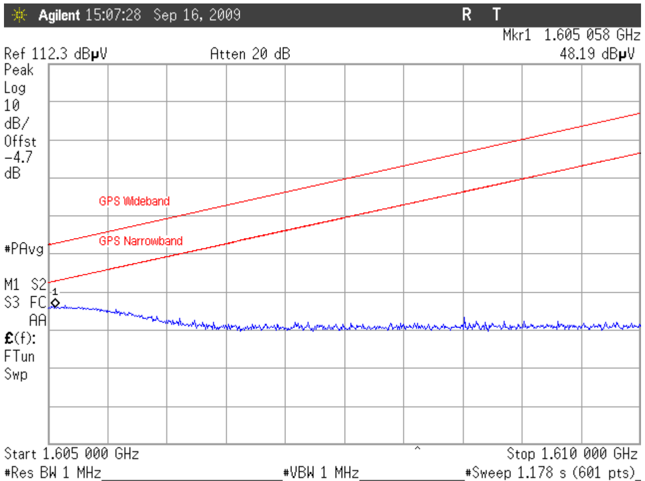
Figure 11: GPS Band Emissions Low Channel, 1605 – 1610MHz Vertical Antenna Polarity
