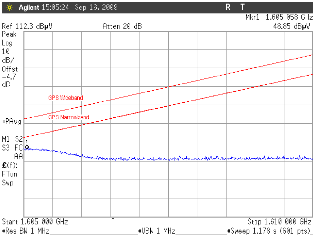
Figure 13: GPS Band Emissions Low Channel, 1605 – 1610MHz Horizontal Antenna Polarity
