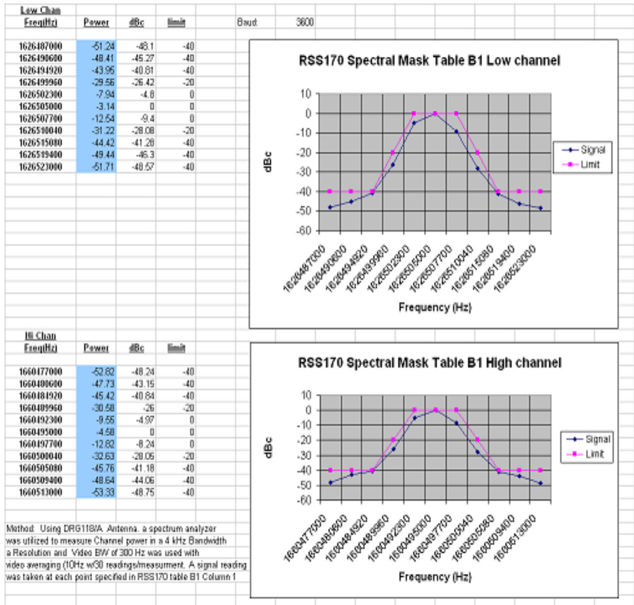
Figure 7: Out-of-Band Emissions to Table B1
