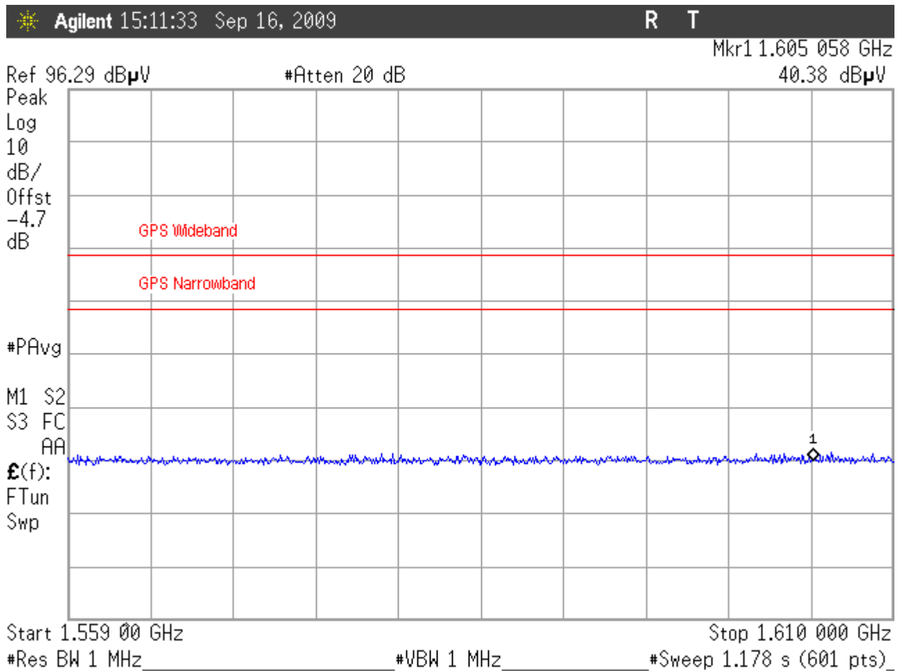
Figure 18: GPS Band Emission, Carrier Off, Mid Channel, 1559 – 1610MHz
