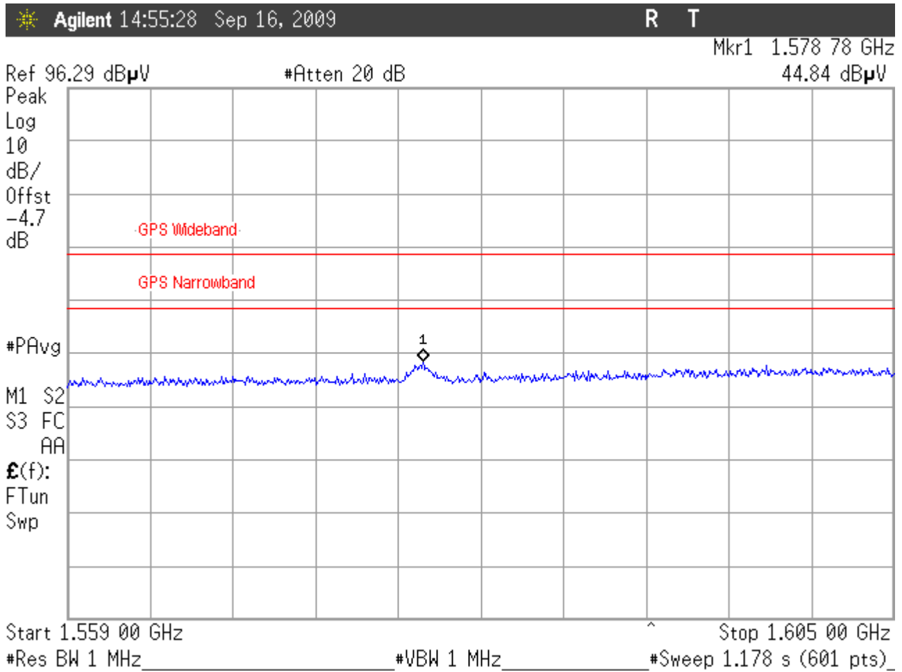
Figure 19: GPS Band Emissions High Channel, 1559 – 1605MHz Vertical Antenna Polarity
