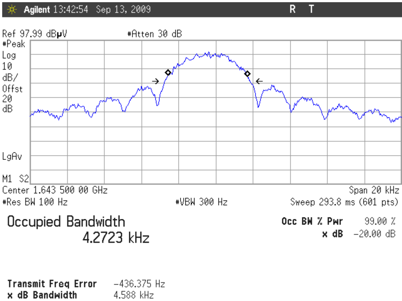
Figure 3: Occupied Bandwidth, Mid Channel, TX @ 1643.5MHz
