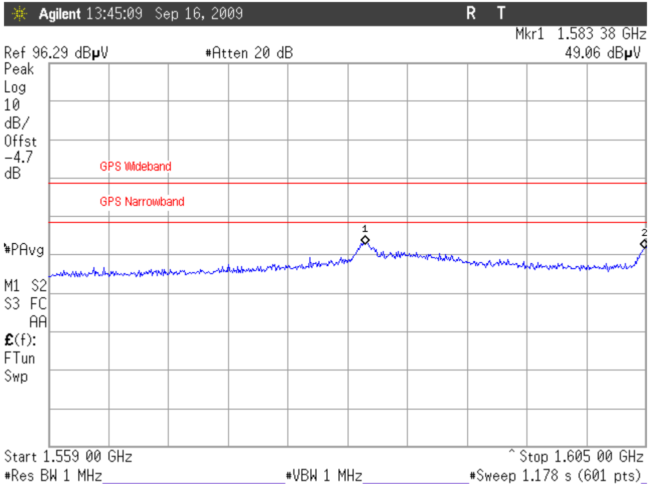
Figure 10: GPS Band Emissions Low Channel, 1559 – 1605MHz Vertical Antenna Polarity
