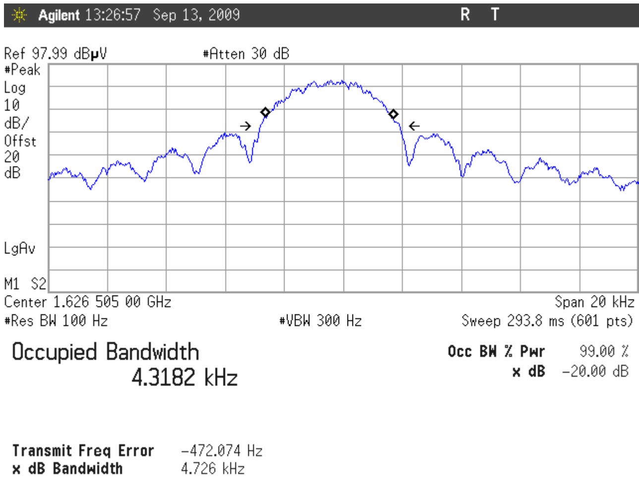
Figure 2: Occupied Bandwidth, Low Channel, TX @ 1626.505MHz
