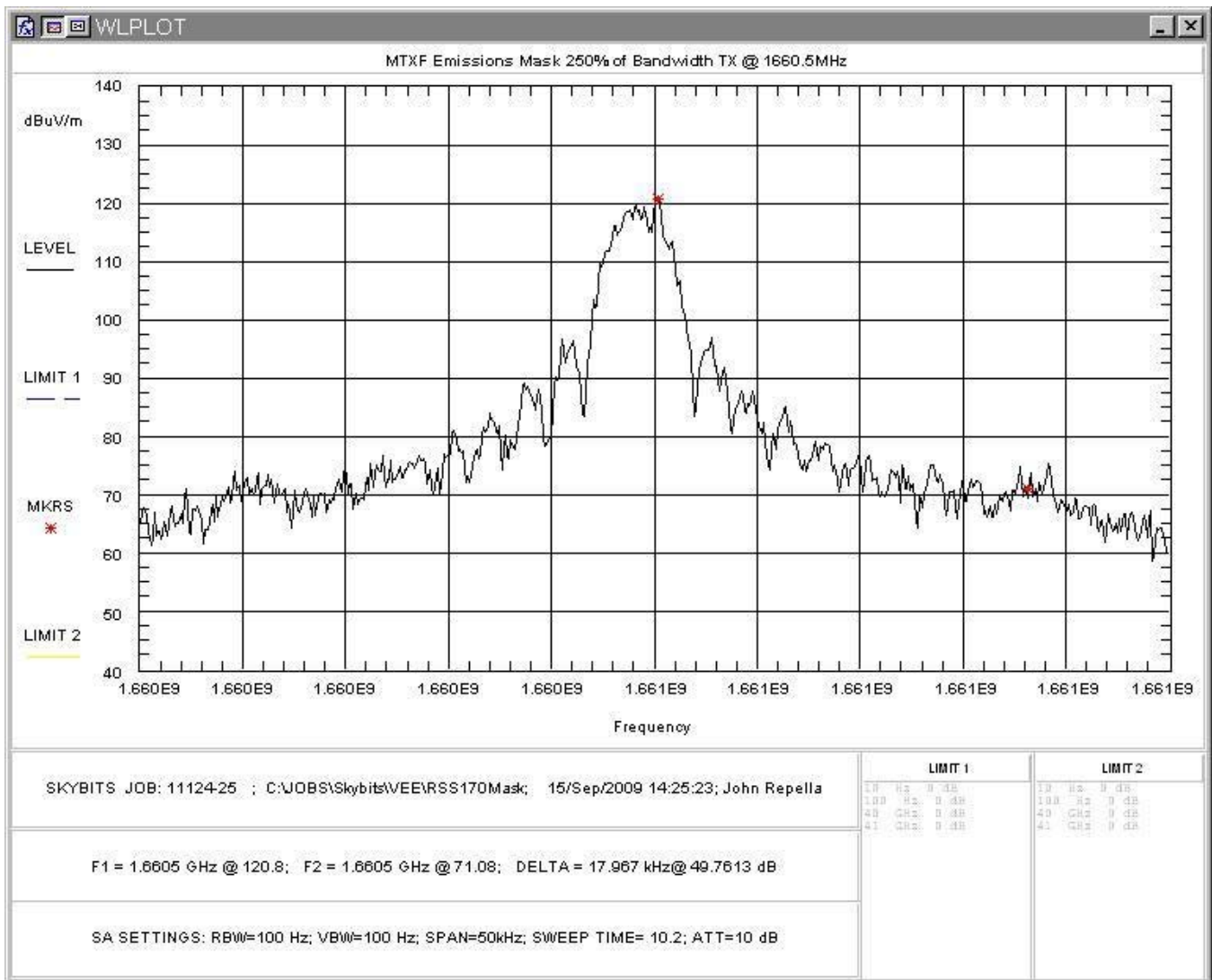
Figure 9: Spectrum Plot, High Channel @ +/-250% of BW
