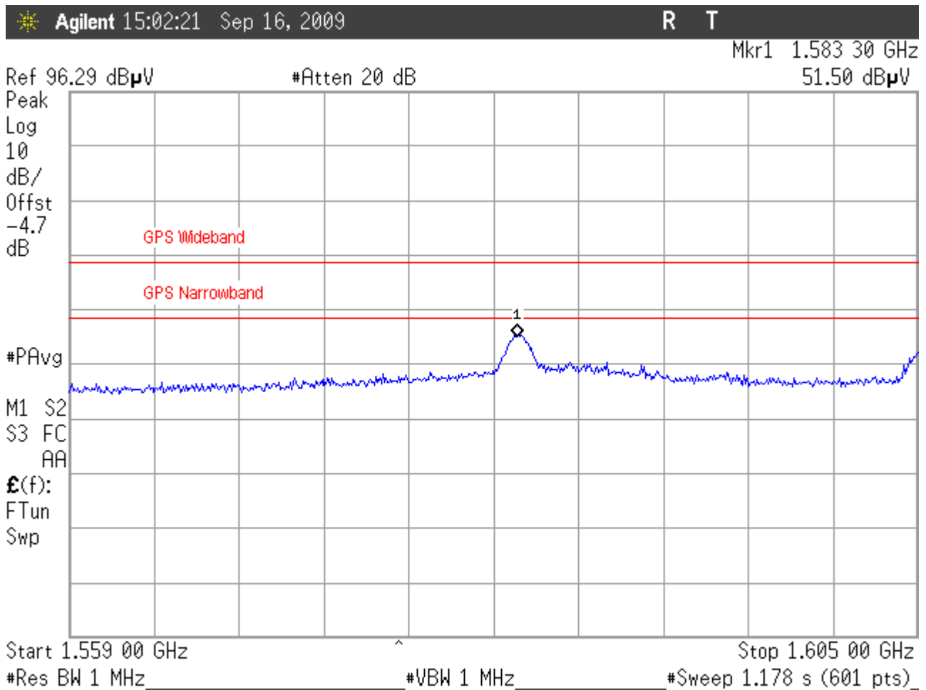
Figure 12: GPS Band Emissions Low Channel, 1559 – 1605MHz Horizontal Antenna Polarity
