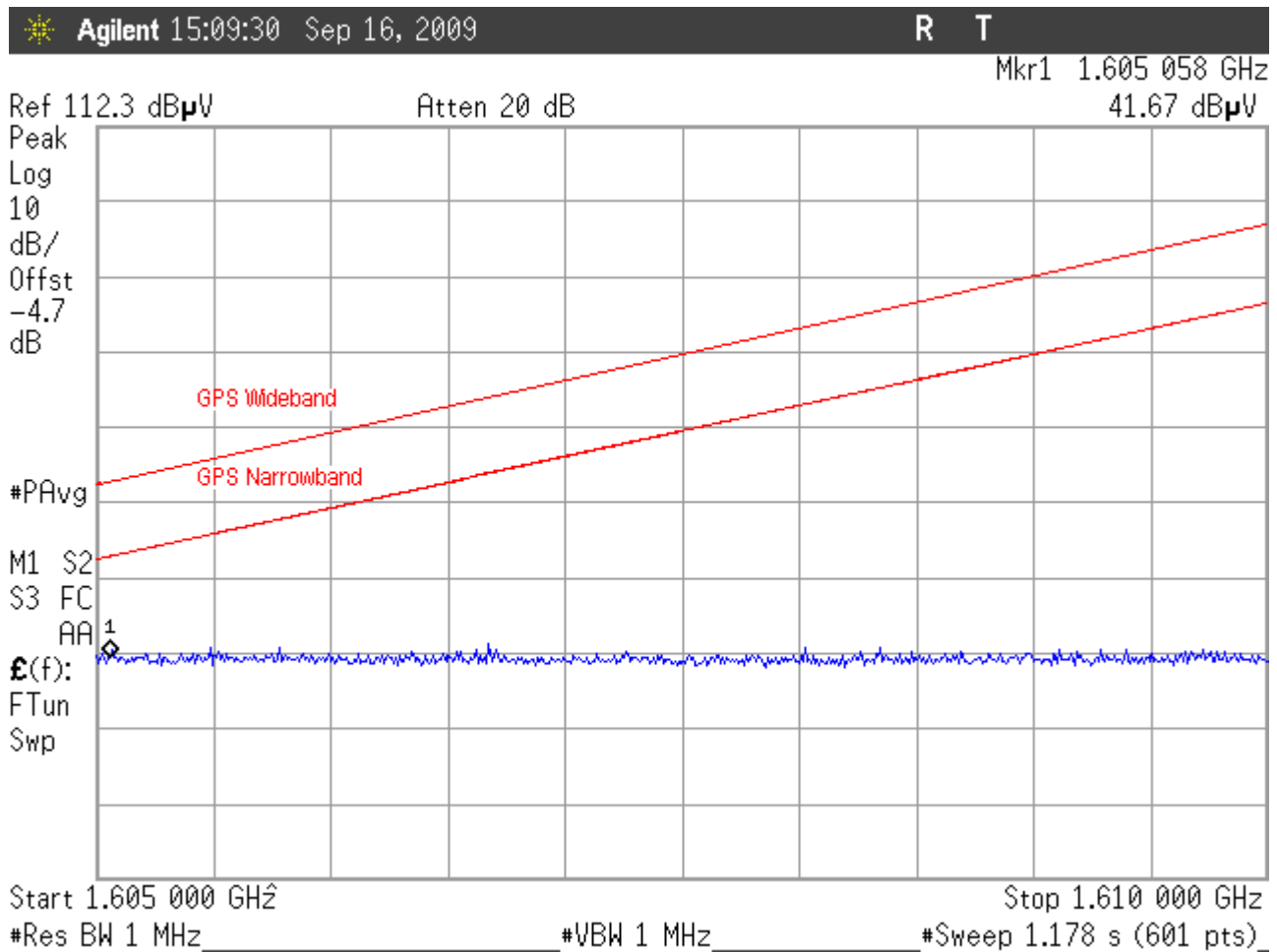
Figure 15: GPS Band Emissions Middle Channel, 1605 – 1610MHz, Vertical Antenna Polarity
