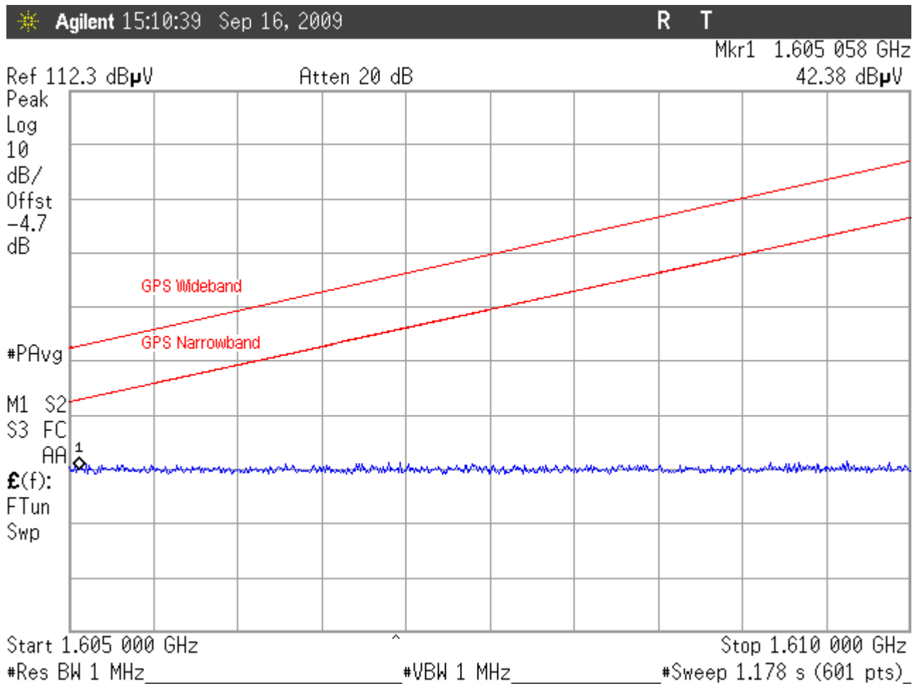
Figure 17: GPS Band Emissions Middle Channel, 1605 – 1610MHz, Horizontal Antenna Polarity
