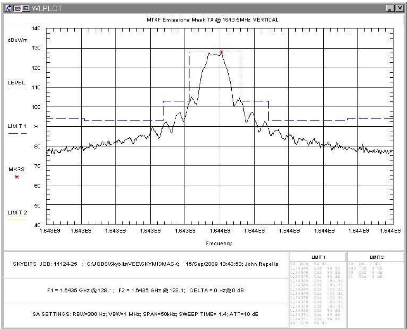
Figure 5: FCC Part 25.202(f) Emissions Mask, Vertical Polarity
