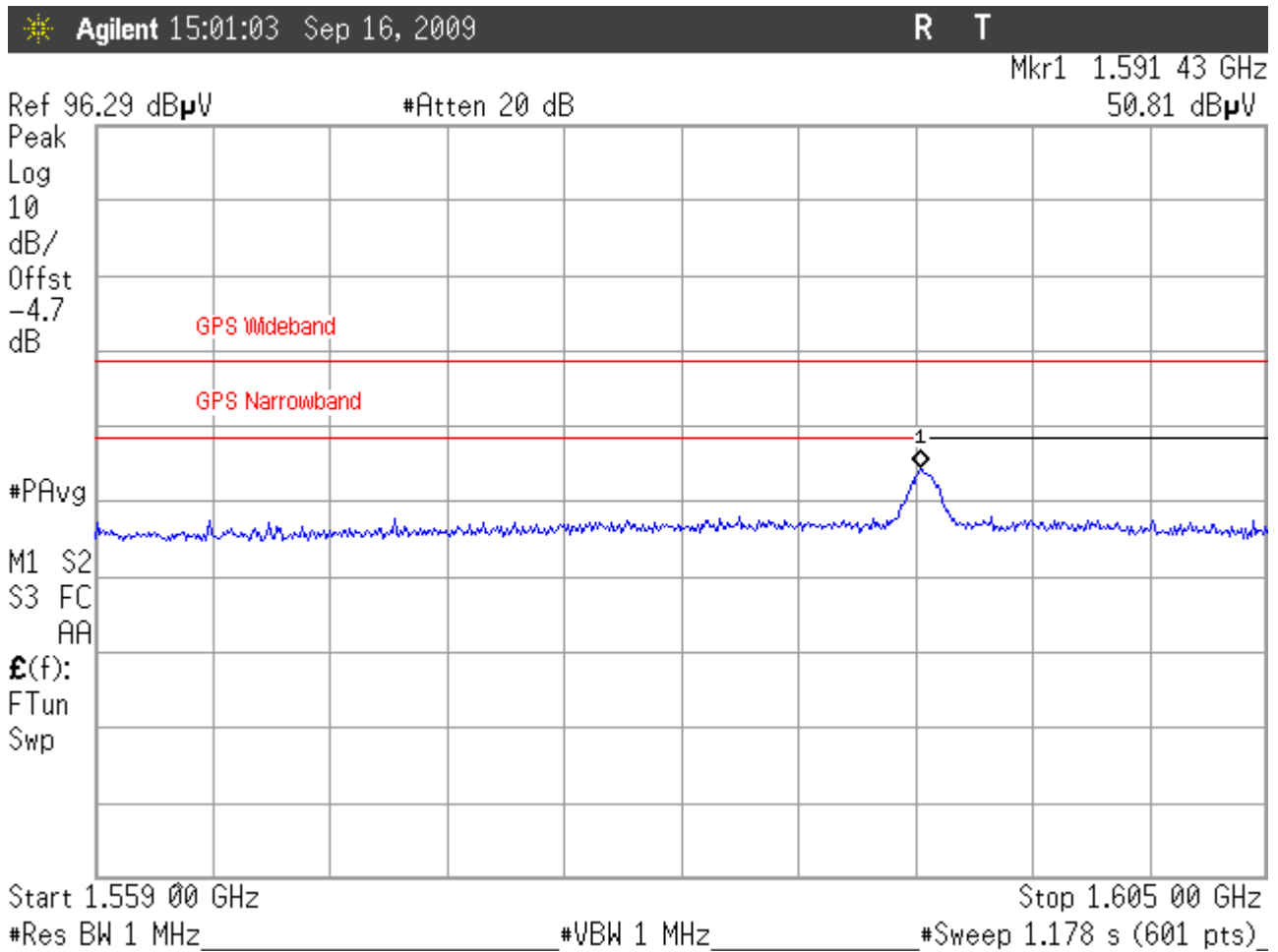
Figure 16: GPS Band Emissions Middle Channel, 1559 – 1605MHz, Horizontal Antenna Polarity
