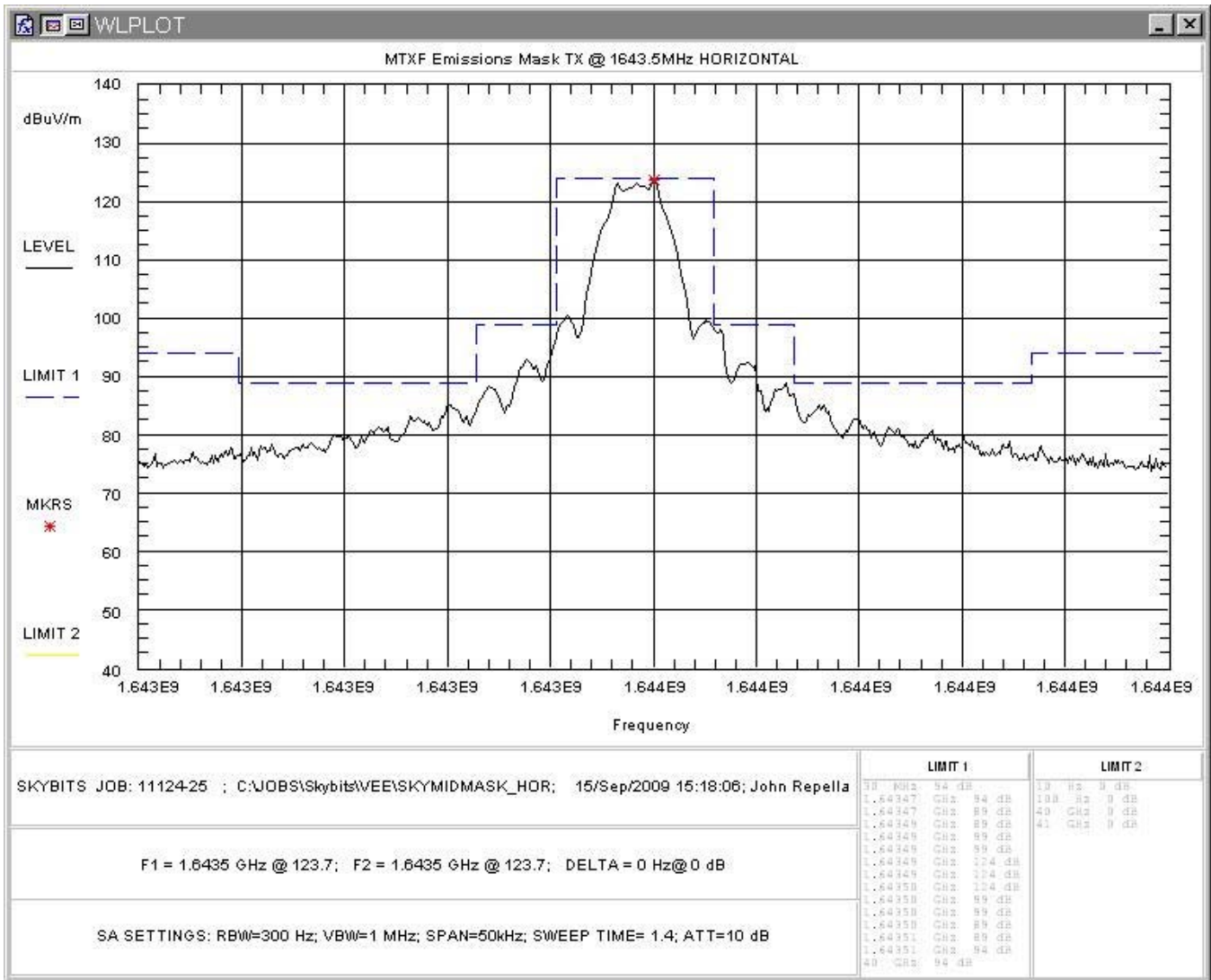
Figure 6: FCC Part 25.202(f) Emissions Mask, Horizontal Polarity
