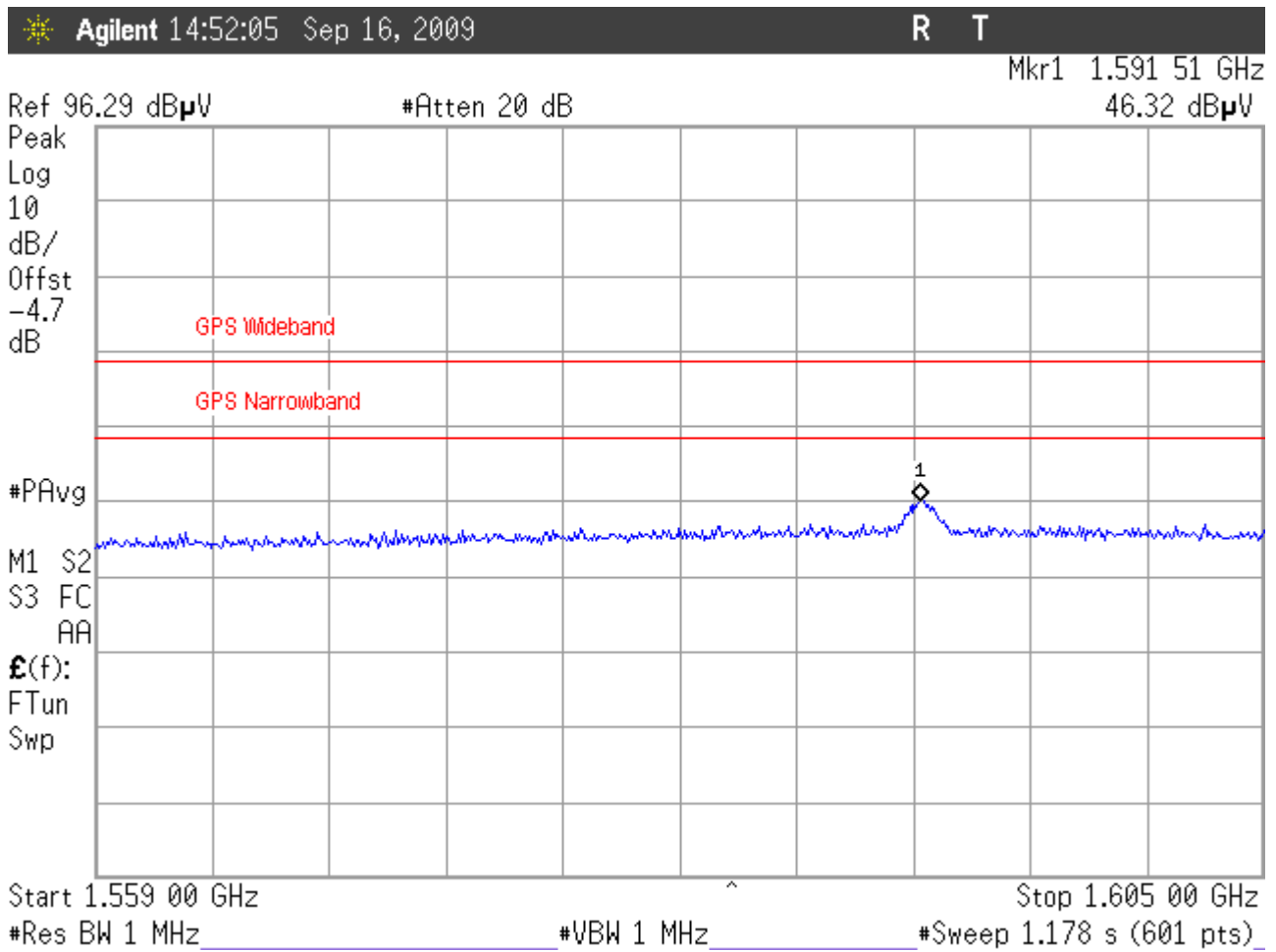
Figure 14: GPS Band Emissions Middle Channel, 1559 – 1605MHz, Vertical Antenna Polarity
