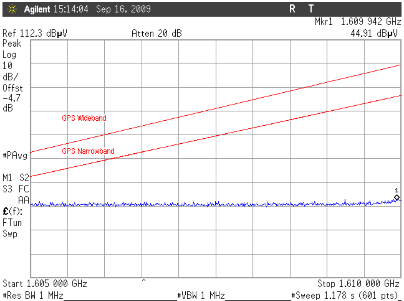
Figure 20: GPS Band Emissions High Channel, 1605 – 1610MHz Vertical Antenna Polarity
