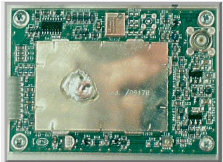
Fig. # 7. CHANNEL R.F. OSCILLATOR & PHASE-LOCKED LOOP CIRCUIT CARD.
