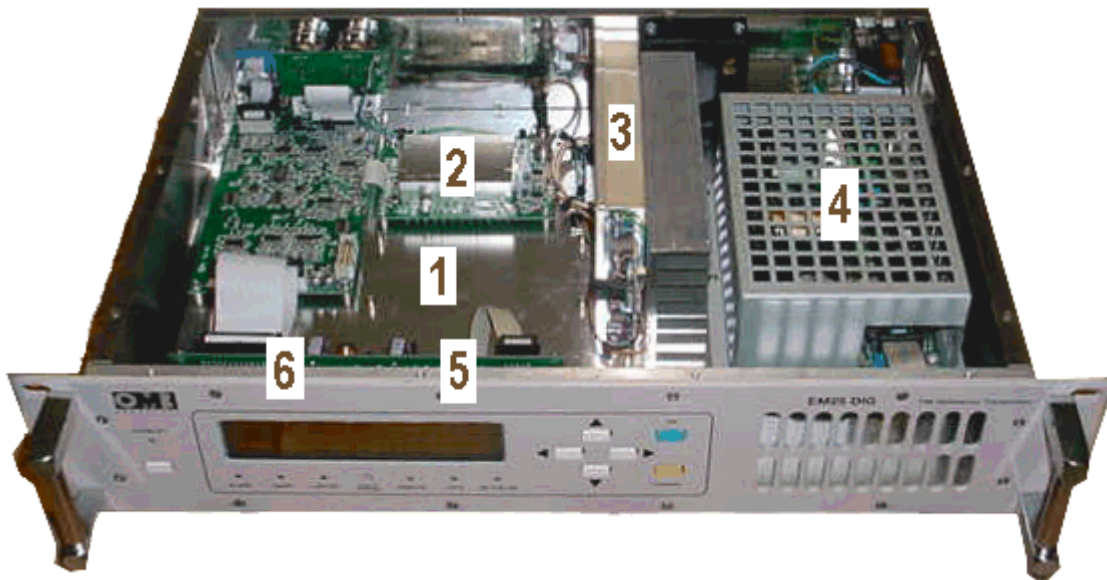
Fig.#5.EM-25 DIG F.M.MODULADOR-EXCITER.UPPER VIEW WITH COVER REMOVED.
