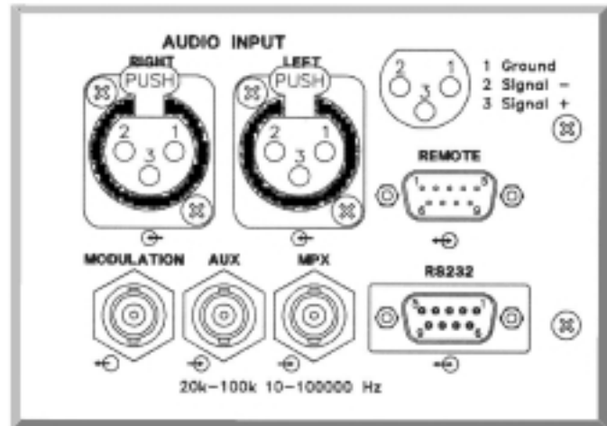
Fig. # 12. CABINET'S CONNECTIONS REAR PANEL
