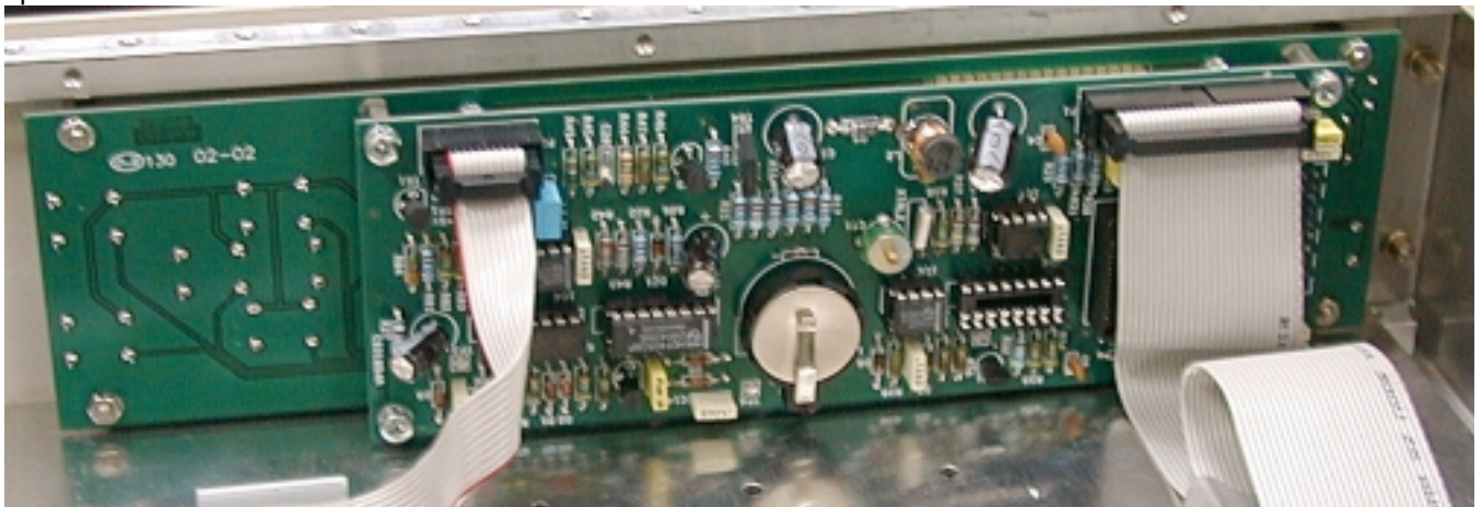
Fig. # 8.- MICROCONTROLLER UNIT AND DISPLAY BOARD
