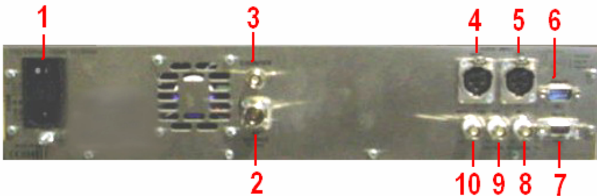
Fig.#3. EM-25 DIG F.M.MODULADOR-EXCITER. REAR PANEL.
