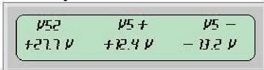
Fig. # 24. INTERNAL POWER SUPPLY VOLTAGES MENU. (No. 08)
