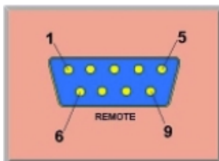
Fig.#4.REMOTE CONNECTOR PINS
