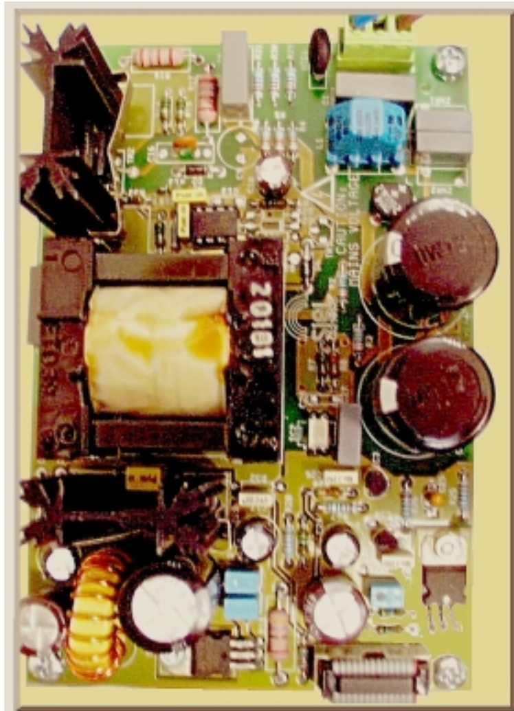
Fig. # 10. SWITCHING POWER SUPPLY UNIT. PRINTED CIRCUIT CARD.
