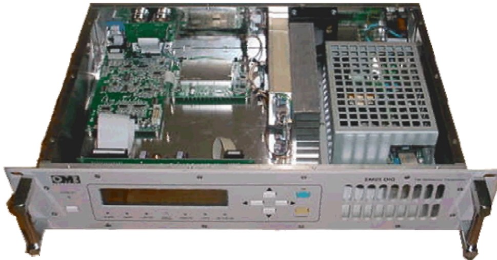
Fig.#1. EXTERNAL VIEW OF EM-25 DIG MODULATOR /EXCITER
