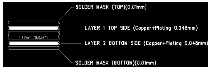
Figure 24: Example stack-up
