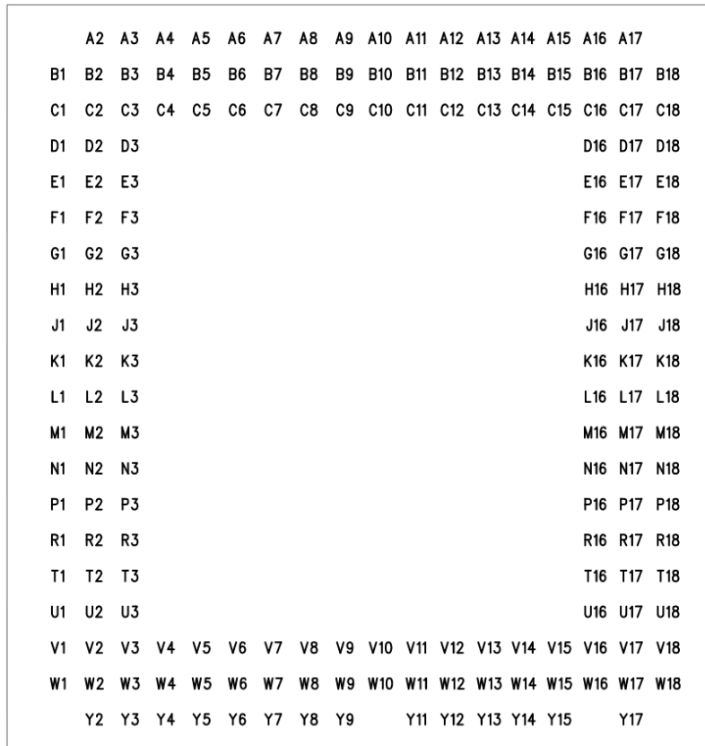
Figure 26: Pin Numbering Diagram Bottom view
