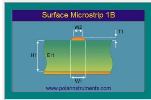
Figure 23: Micro-strip trace parameters
