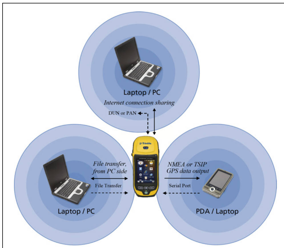
Figure 6.2 GeoExplorer 6000 series handheld Bluetooth host connections
