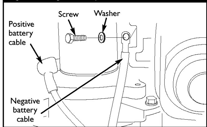
Figure 1 — Negative Battery Connection
