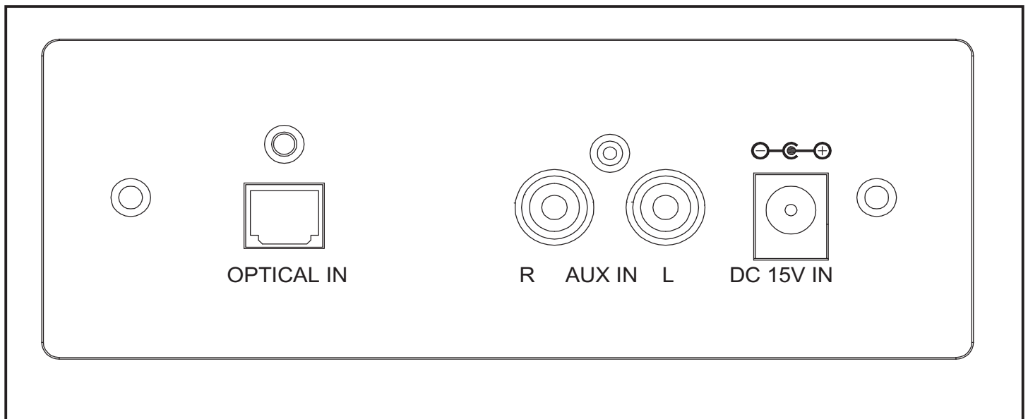
Fig.1 Back Panel
