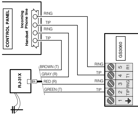
Fig. 3 - Telephone Connection
